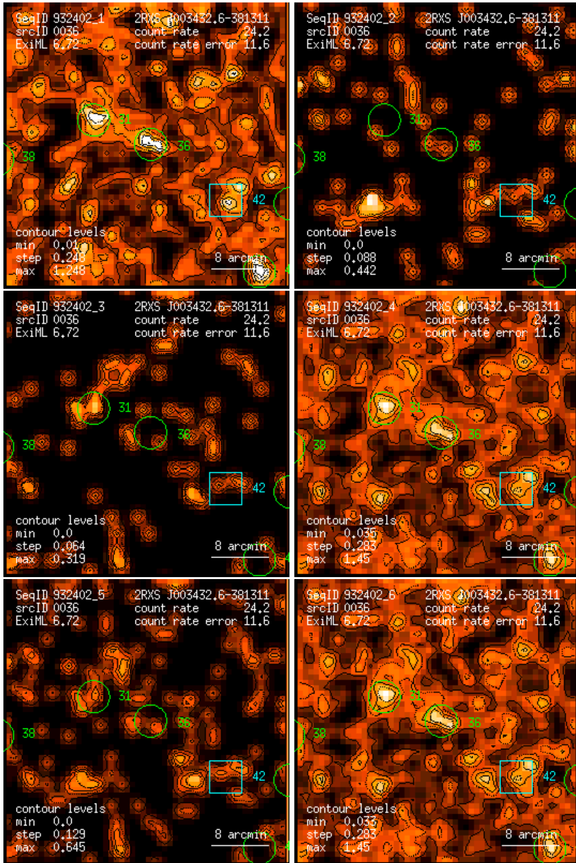
Figure 36: RASS 932402: detection 0036: band rate images, Gaussian filter: (1) PSPC channels 11 – 41, (2) 52 – 90, (3) 91 – 201, (4) 11 – 235, (5) 52 – 201, (6) 11 – 201. Broad band rates in counts/ks. Band rate contour levels in counts/ks/arcmin 2 .
