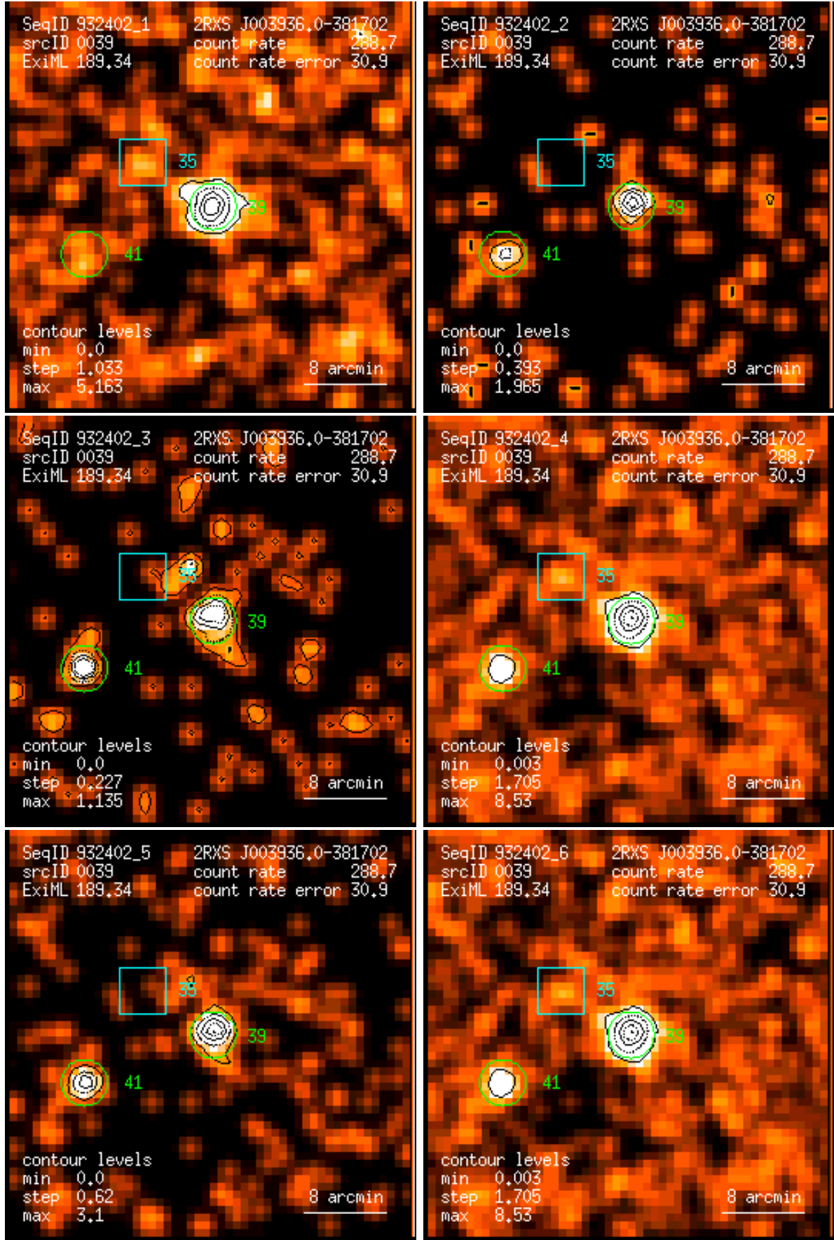
Figure 39: RASS 932402: detection 0039: band rate images, Gaussian filter: (1) PSPC channels 11 – 41, (2) 52 – 90, (3) 91 – 201, (4) 11 – 235, (5) 52 – 201, (6) 11 – 201. Broad band rates in counts/ks. Band rate contour levels in counts/ks/arcmin 2 .
