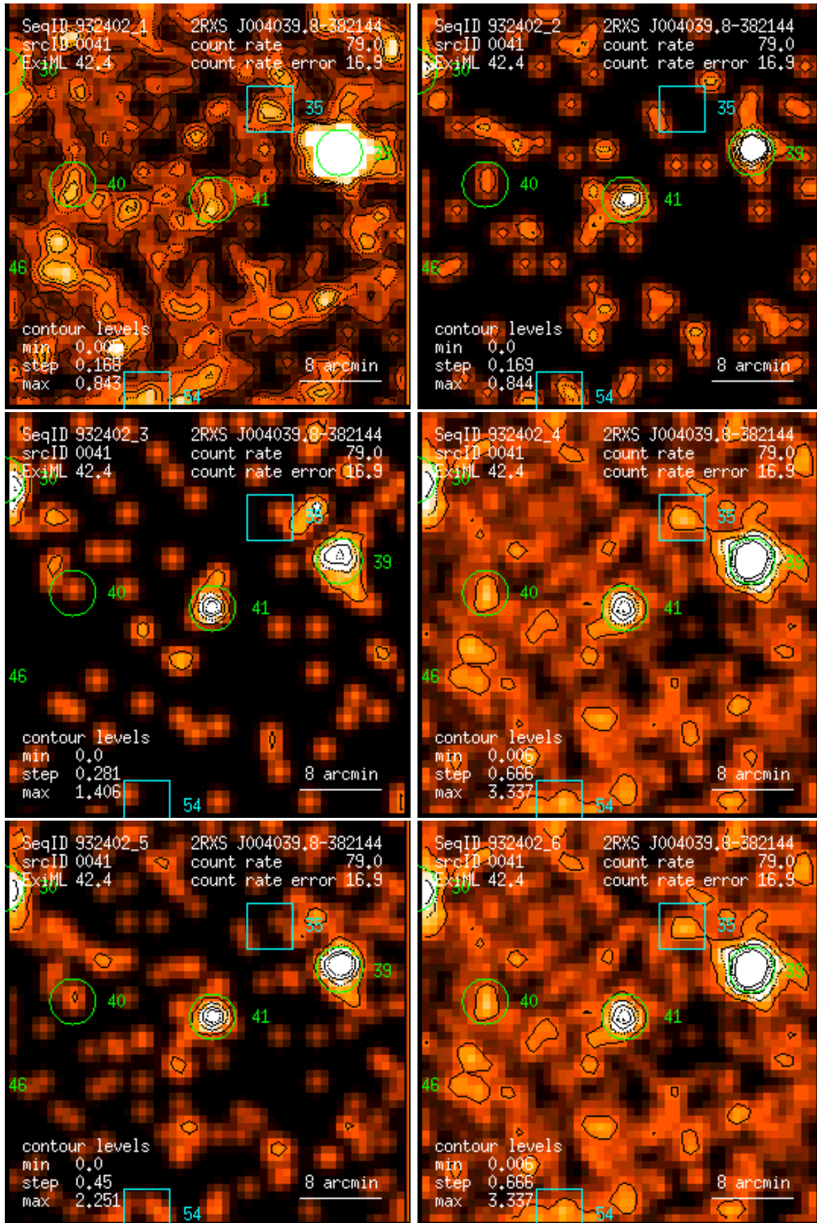
Figure 41: RASS 932402: detection 0041: band rate images, Gaussian filter: (1) PSPC channels 11 – 41, (2) 52 – 90, (3) 91 – 201, (4) 11 – 235, (5) 52 – 201, (6) 11 – 201. Broad band rates in counts/ks. Band rate contour levels in counts/ks/arcmin 2 .
