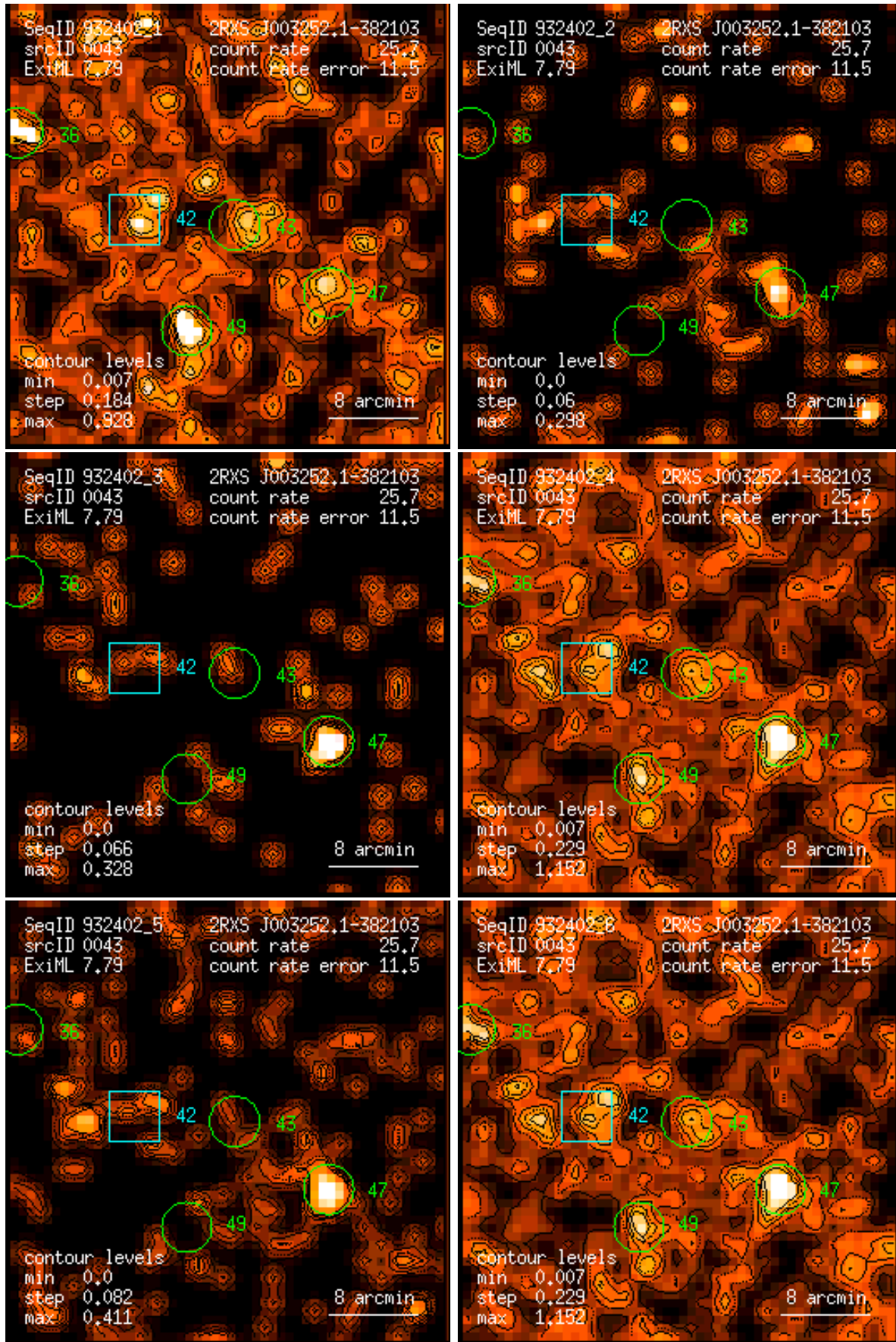
Figure 43: RASS 932402: detection 0043: band rate images, Gaussian filter: (1) PSPC channels 11 – 41, (2) 52 – 90, (3) 91 – 201, (4) 11 – 235, (5) 52 – 201, (6) 11 – 201. Broad band rates in counts/ks. Band rate contour levels in counts/ks/arcmin 2 .
