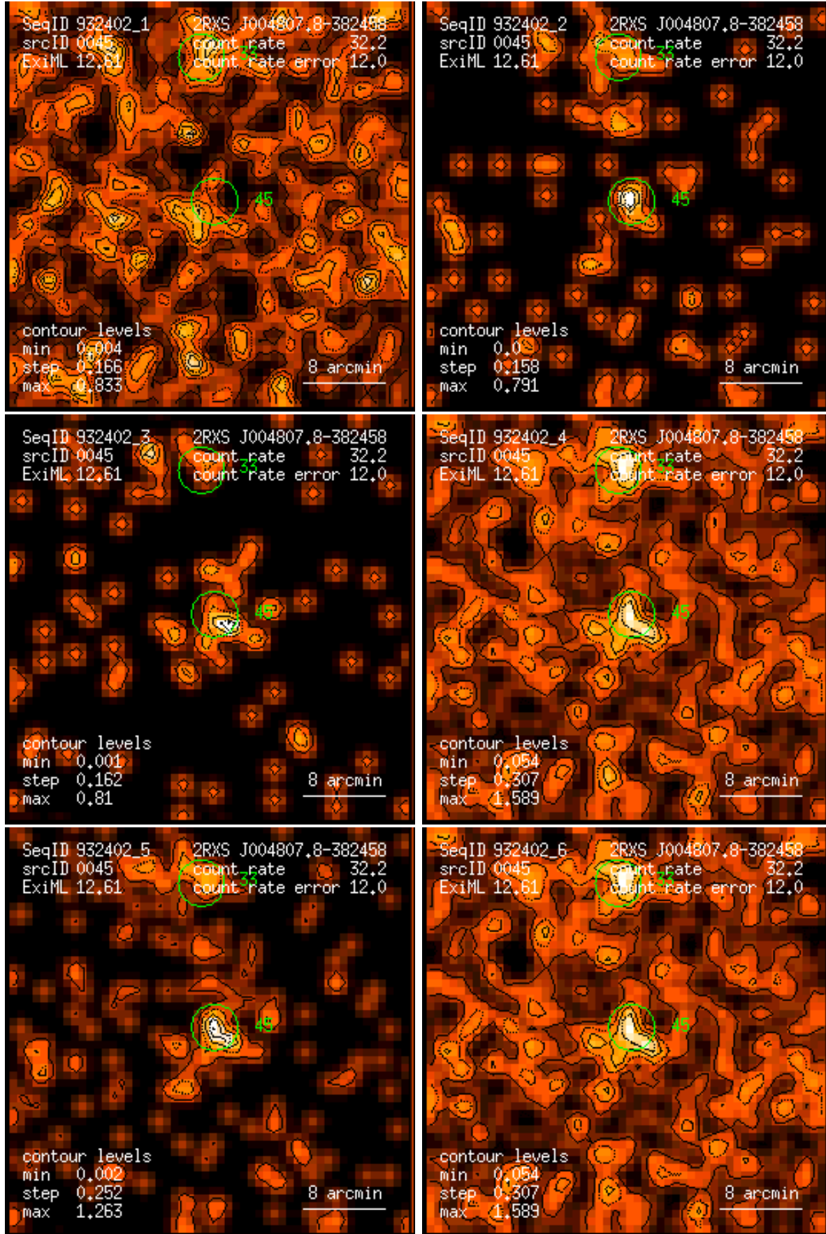
Figure 45: RASS 932402: detection 0045: band rate images, Gaussian filter: (1) PSPC channels 11 – 41, (2) 52 – 90, (3) 91 – 201, (4) 11 – 235, (5) 52 – 201, (6) 11 – 201. Broad band rates in counts/ks. Band rate contour levels in counts/ks/arcmin 2 .
