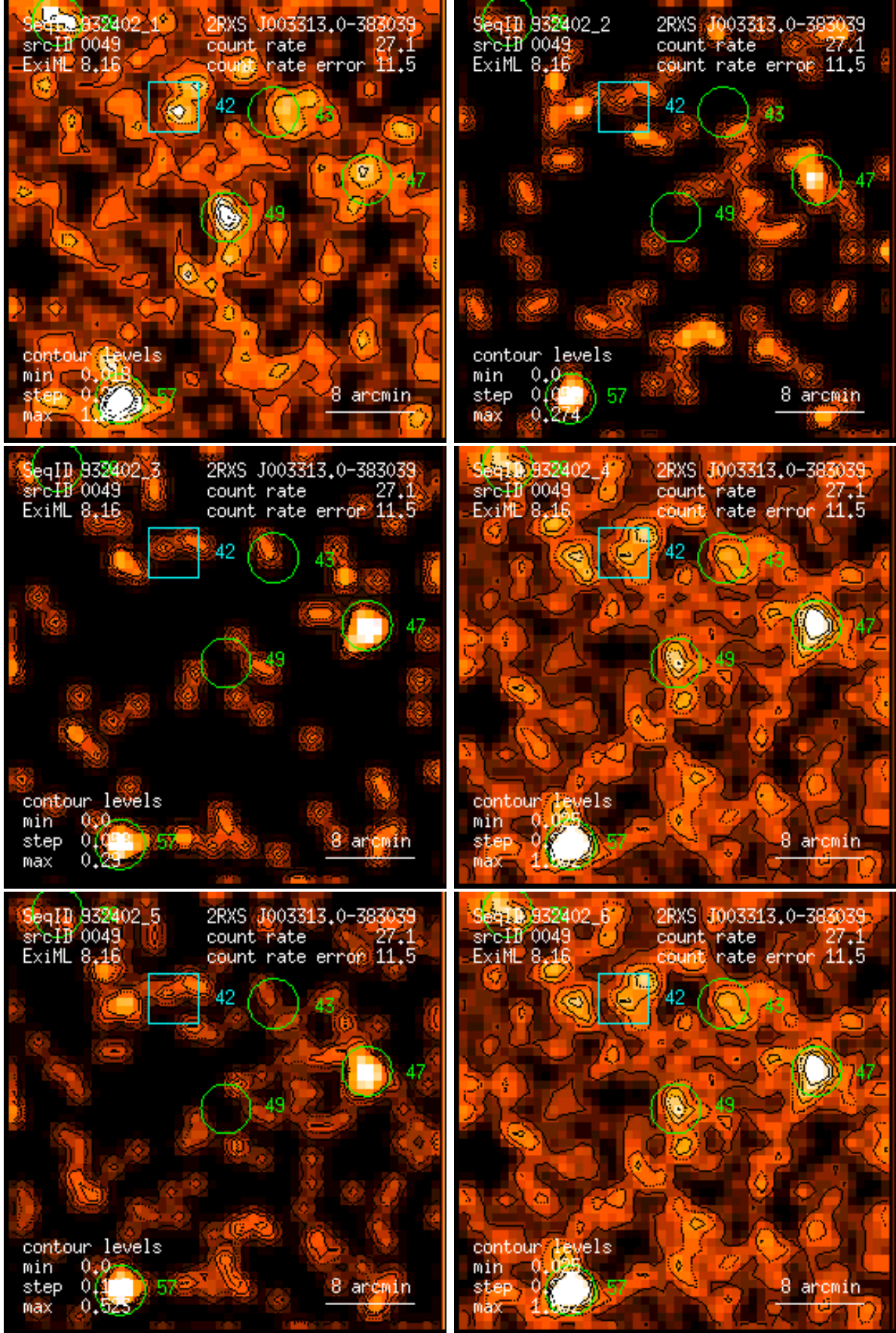
Figure 49: RASS 932402: detection 0049: band rate images, Gaussian filter: (1) PSPC channels 11 – 41, (2) 52 – 90, (3) 91 – 201, (4) 11 – 235, (5) 52 – 201, (6) 11 – 201. Broad band rates in counts/ks. Band rate contour levels in counts/ks/arcmin 2 .
