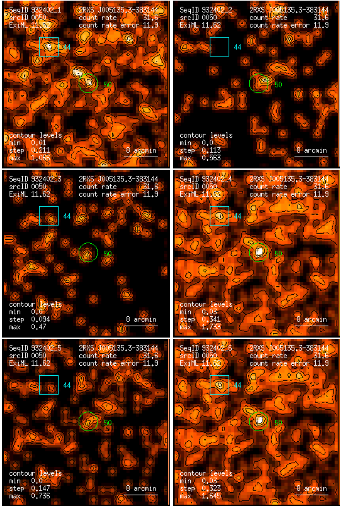
Figure 50: RASS 932402: detection 0050: band rate images, Gaussian filter: (1) PSPC channels 11 – 41, (2) 52 – 90, (3) 91 – 201, (4) 11 – 235, (5) 52 – 201, (6) 11 – 201. Broad band rates in counts/ks. Band rate contour levels in counts/ks/arcmin 2 .
