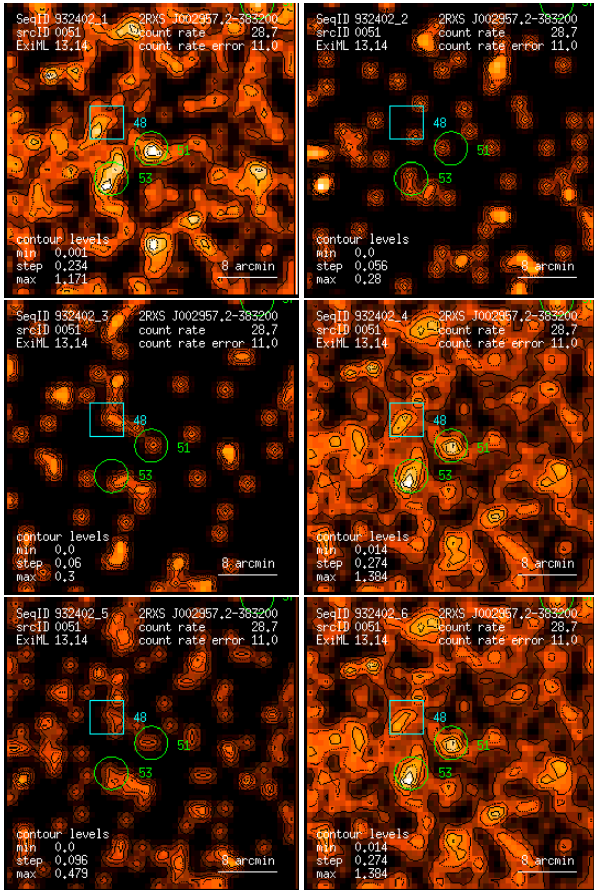
Figure 51: RASS 932402: detection 0051: band rate images, Gaussian filter: (1) PSPC channels 11 – 41, (2) 52 – 90, (3) 91 – 201, (4) 11 – 235, (5) 52 – 201, (6) 11 – 201. Broad band rates in counts/ks. Band rate contour levels in counts/ks/arcmin 2 .
