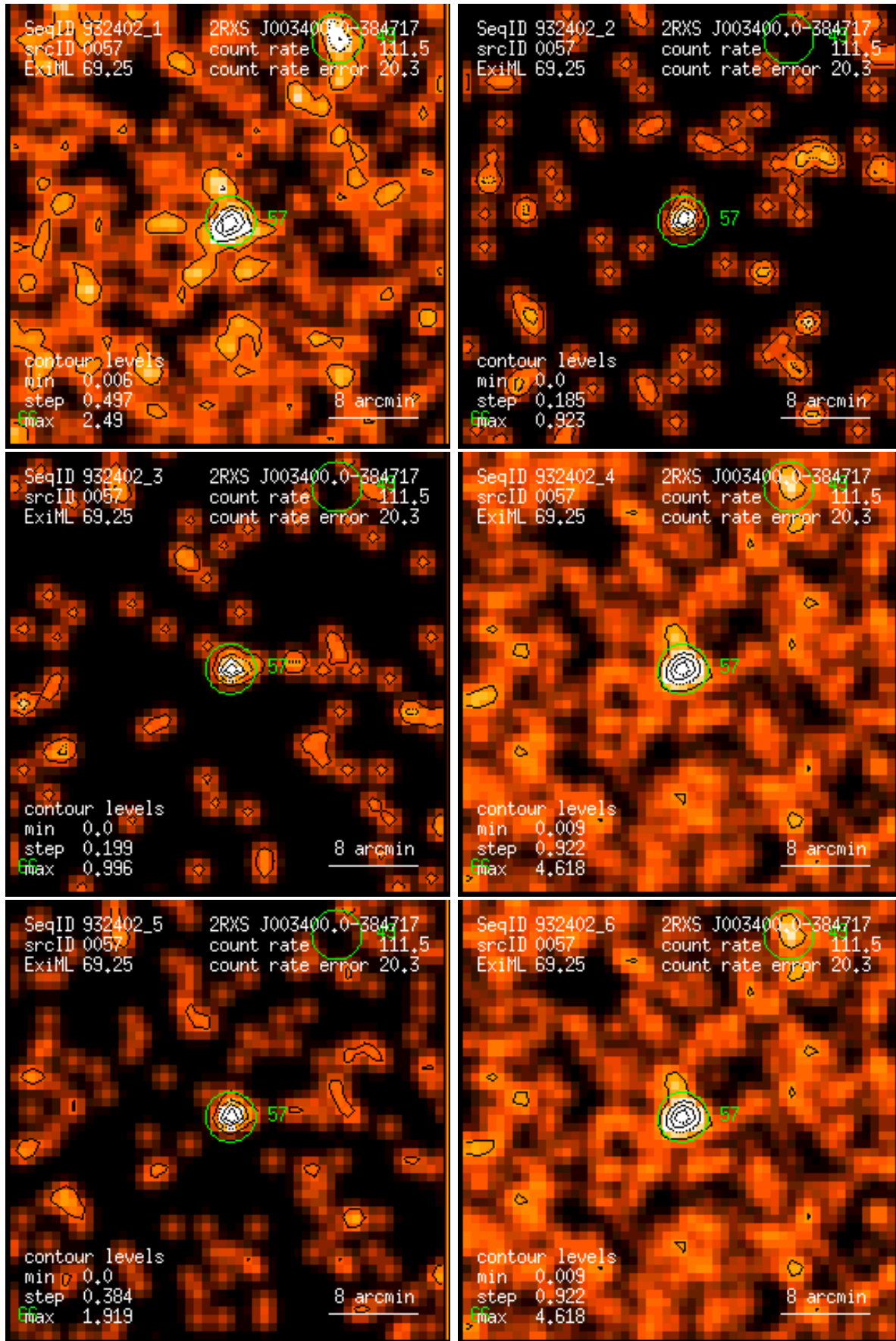
Figure 57: RASS 932402: detection 0057: band rate images, Gaussian filter: (1) PSPC channels 11 – 41, (2) 52 – 90, (3) 91 – 201, (4) 11 – 235, (5) 52 – 201, (6) 11 – 201. Broad band rates in counts/ks. Band rate contour levels in counts/ks/arcmin 2 .
