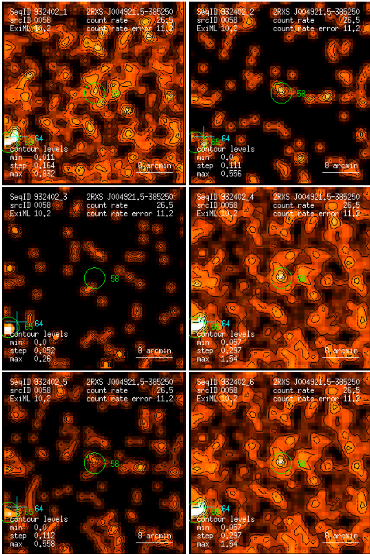
Figure 58: RASS 932402: detection 0058: band rate images, Gaussian filter: (1) PSPC channels 11 – 41, (2) 52 – 90, (3) 91 – 201, (4) 11 – 235, (5) 52 – 201, (6) 11 – 201. Broad band rates in counts/ks. Band rate contour levels in counts/ks/arcmin 2 .
