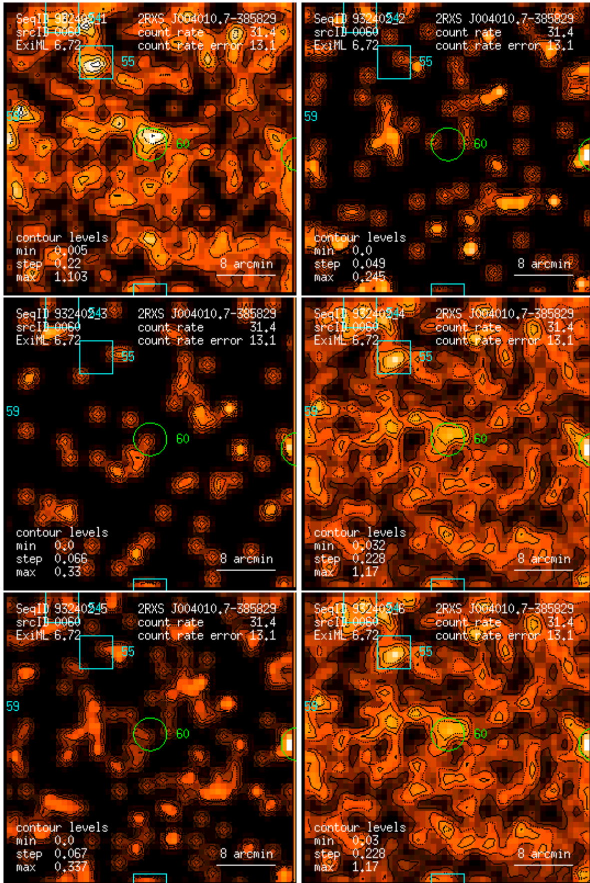
Figure 60: RASS 932402: detection 0060: band rate images, Gaussian filter: (1) PSPC channels 11 – 41, (2) 52 – 90, (3) 91 – 201, (4) 11 – 235, (5) 52 – 201, (6) 11 – 201. Broad band rates in counts/ks. Band rate contour levels in counts/ks/arcmin 2 .
