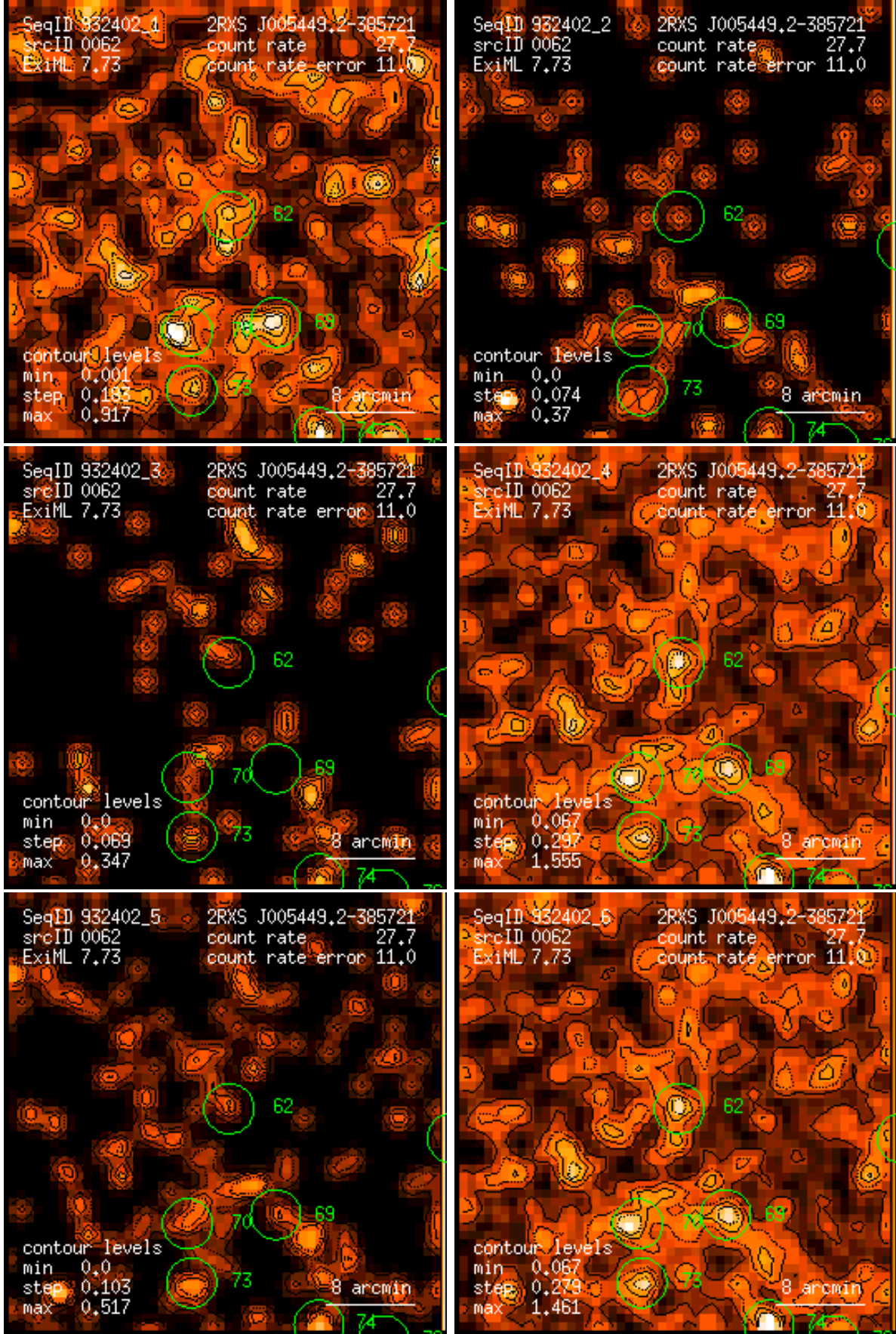
Figure 62: RASS 932402: detection 0062: band rate images, Gaussian filter: (1) PSPC channels 11 – 41, (2) 52 – 90, (3) 91 – 201, (4) 11 – 235, (5) 52 – 201, (6) 11 – 201. Broad band rates in counts/ks. Band rate contour levels in counts/ks/arcmin 2 .
