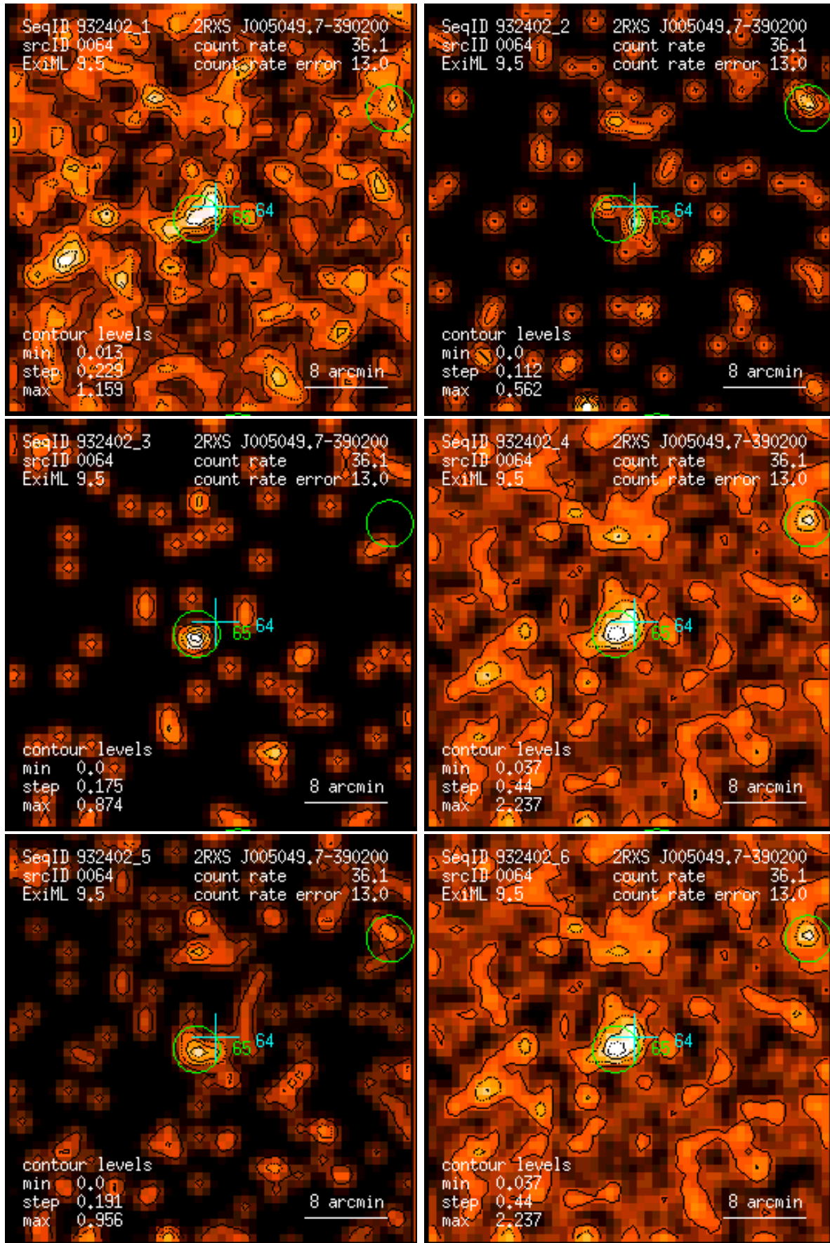
Figure 64: RASS 932402: detection 0064: band rate images, Gaussian filter: (1) PSPC channels 11 – 41, (2) 52 – 90, (3) 91 – 201, (4) 11 – 235, (5) 52 – 201, (6) 11 – 201. Broad band rates in counts/ks. Band rate contour levels in counts/ks/arcmin 2 .
