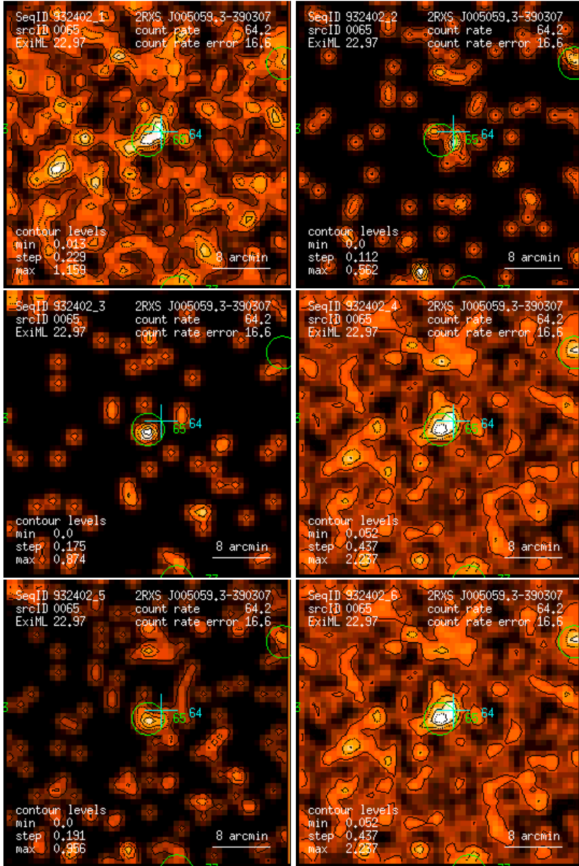
Figure 65: RASS 932402: detection 0065: band rate images, Gaussian filter: (1) PSPC channels 11 – 41, (2) 52 – 90, (3) 91 – 201, (4) 11 – 235, (5) 52 – 201, (6) 11 – 201. Broad band rates in counts/ks. Band rate contour levels in counts/ks/arcmin 2 .
