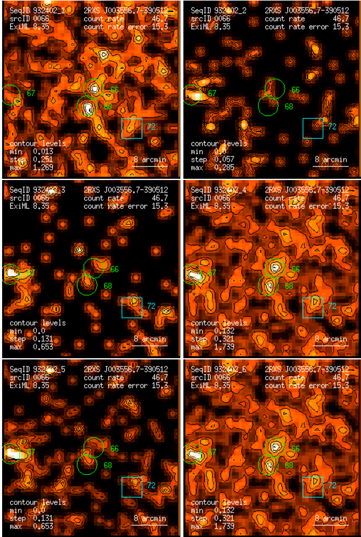
Figure 66: RASS 932402: detection 0066: band rate images, Gaussian filter: (1) PSPC channels 11 – 41, (2) 52 – 90, (3) 91 – 201, (4) 11 – 235, (5) 52 – 201, (6) 11 – 201. Broad band rates in counts/ks. Band rate contour levels in counts/ks/arcmin 2 .
