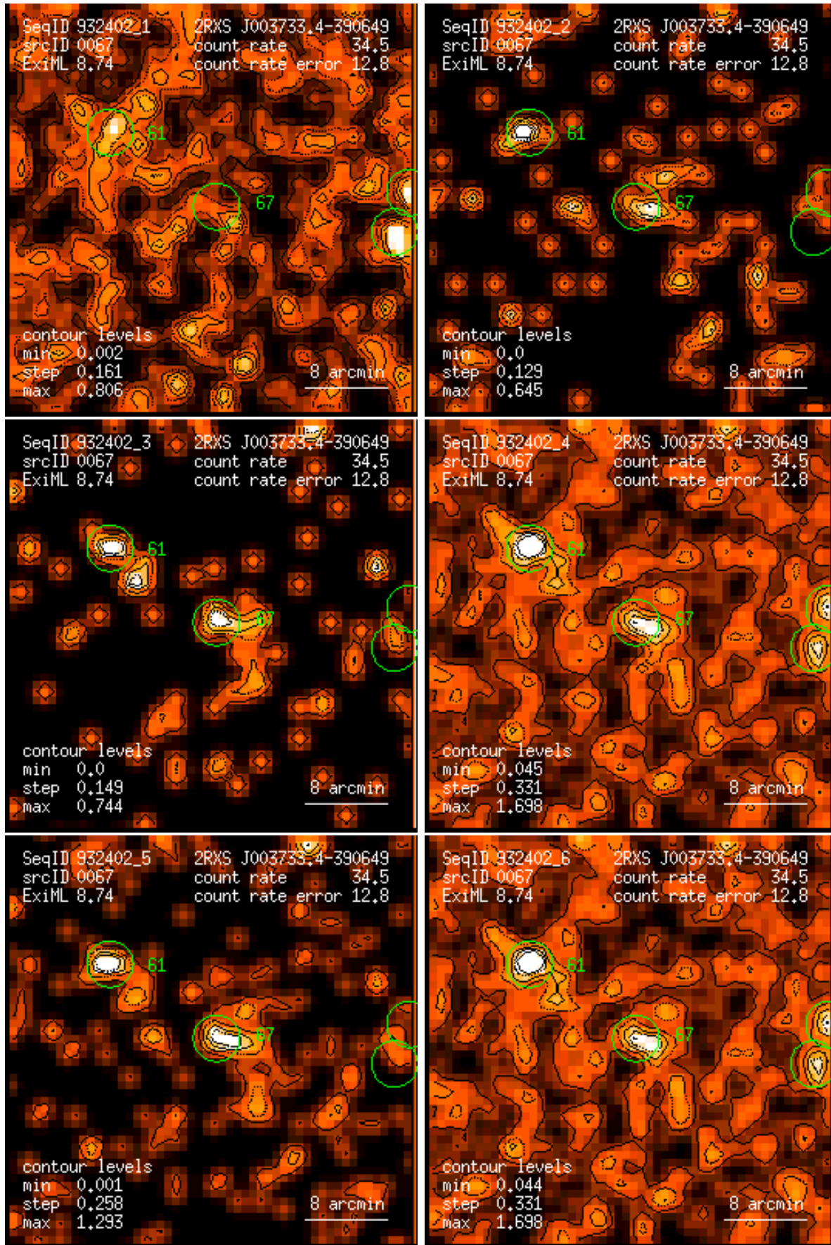
Figure 67: RASS 932402: detection 0067: band rate images, Gaussian filter: (1) PSPC channels 11 – 41, (2) 52 – 90, (3) 91 – 201, (4) 11 – 235, (5) 52 – 201, (6) 11 – 201. Broad band rates in counts/ks. Band rate contour levels in counts/ks/arcmin 2 .
