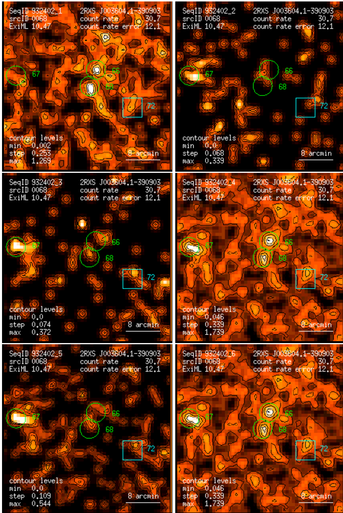
Figure 68: RASS 932402: detection 0068: band rate images, Gaussian filter: (1) PSPC channels 11 – 41, (2) 52 – 90, (3) 91 – 201, (4) 11 – 235, (5) 52 – 201, (6) 11 – 201. Broad band rates in counts/ks. Band rate contour levels in counts/ks/arcmin 2 .
