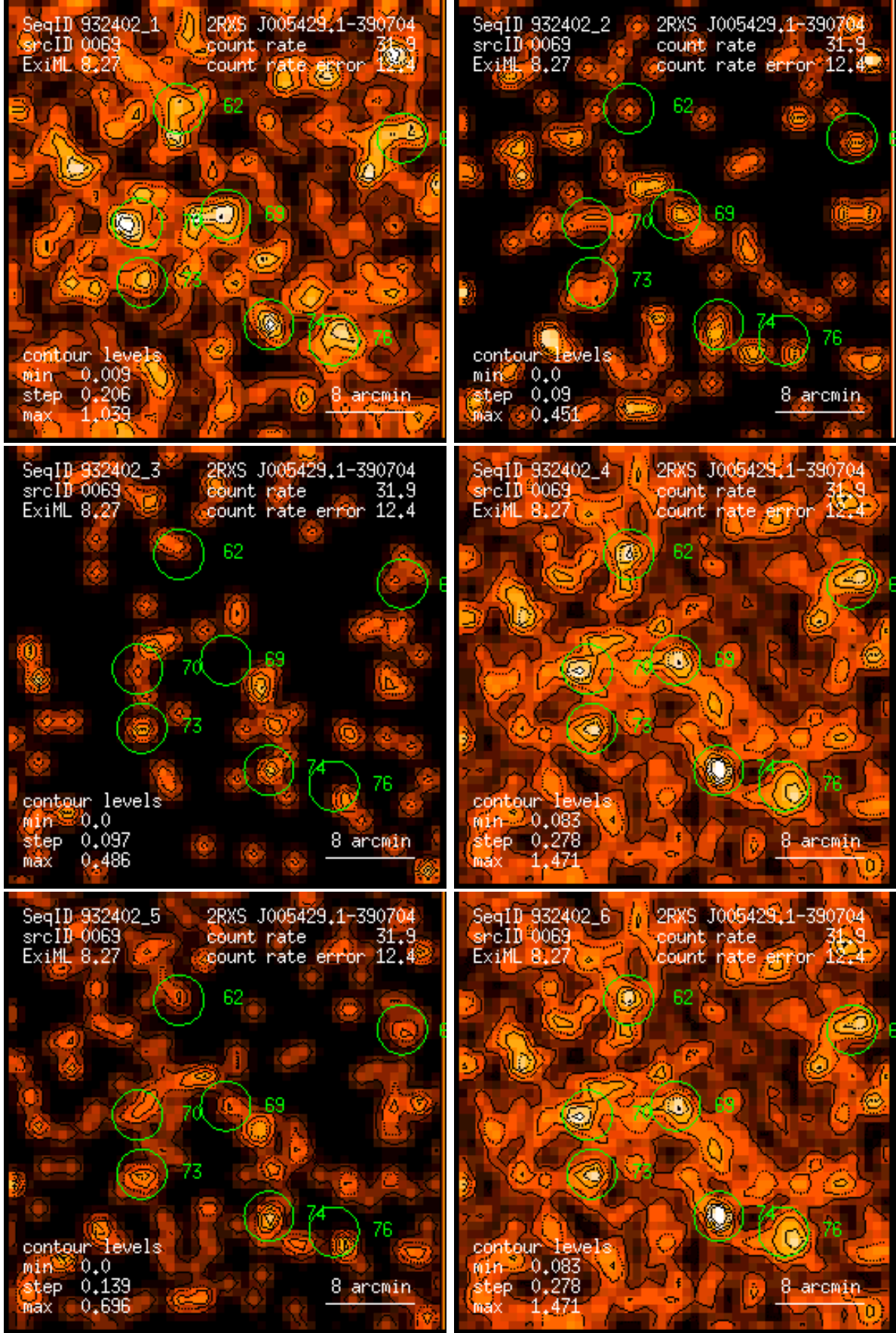
Figure 69: RASS 932402: detection 0069: band rate images, Gaussian filter: (1) PSPC channels 11 – 41, (2) 52 – 90, (3) 91 – 201, (4) 11 – 235, (5) 52 – 201, (6) 11 – 201. Broad band rates in counts/ks. Band rate contour levels in counts/ks/arcmin 2 .
