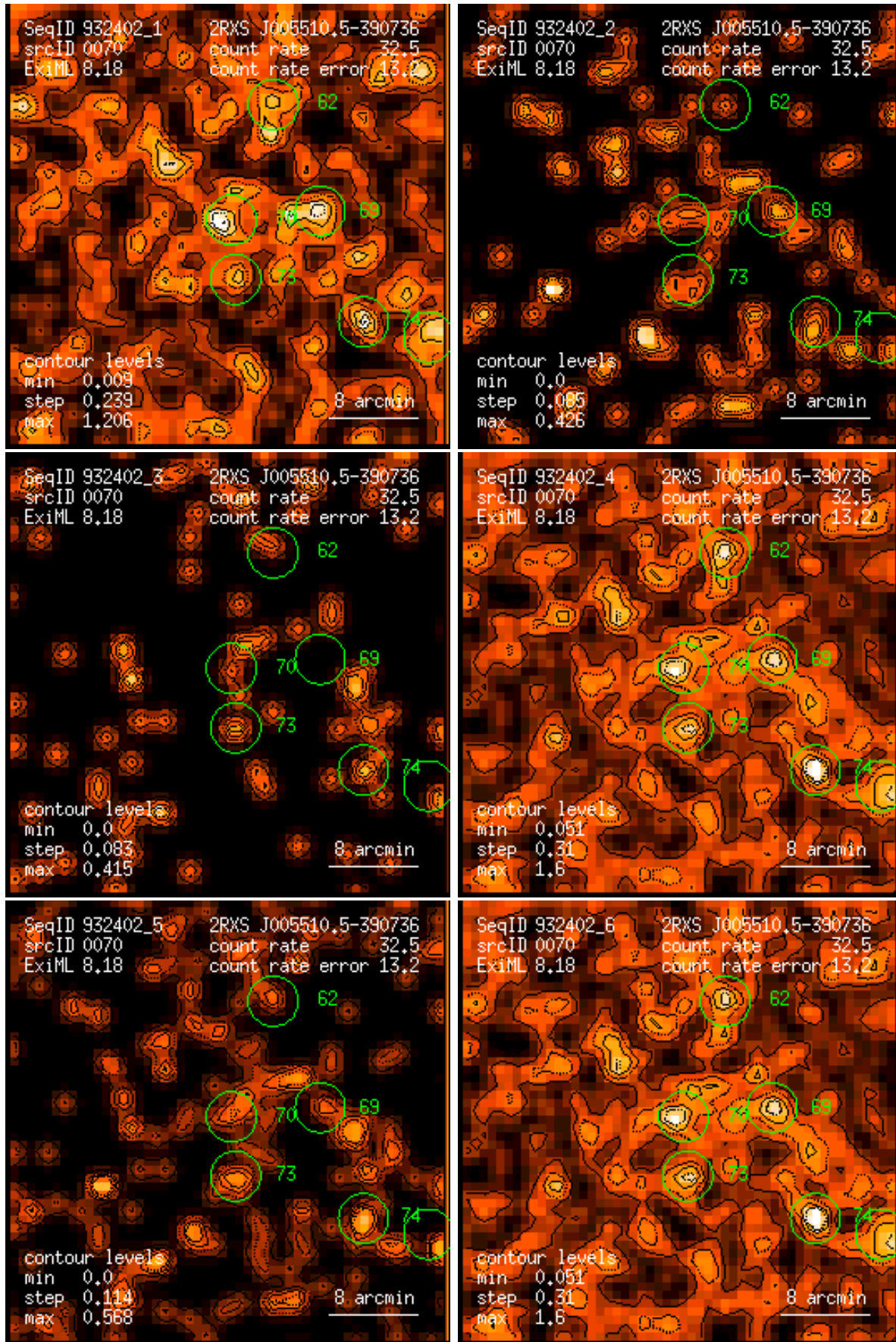
Figure 70: RASS 932402: detection 0070: band rate images, Gaussian filter: (1) PSPC channels 11 – 41, (2) 52 – 90, (3) 91 – 201, (4) 11 – 235, (5) 52 – 201, (6) 11 – 201. Broad band rates in counts/ks. Band rate contour levels in counts/ks/arcmin 2 .
