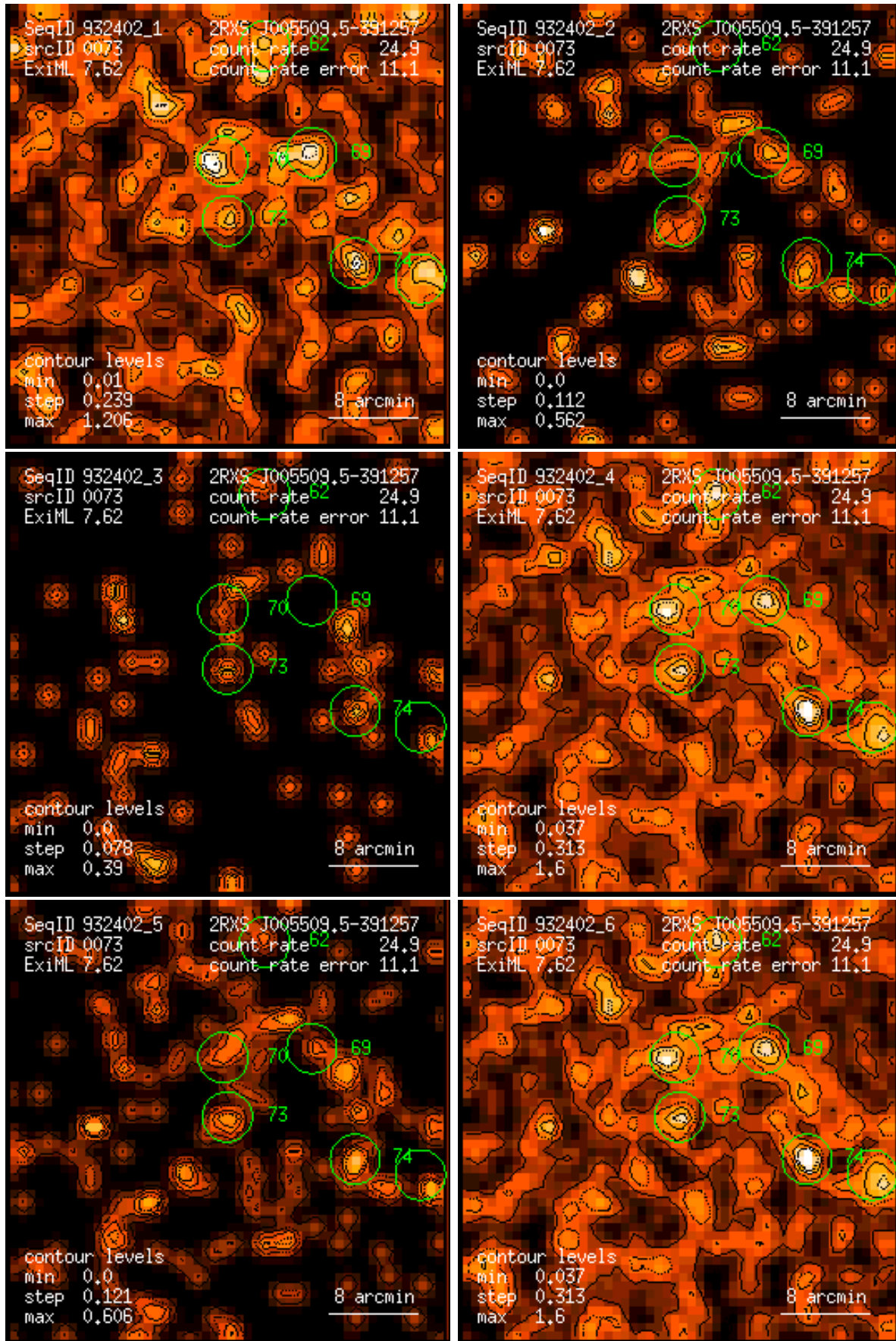
Figure 73: RASS 932402: detection 0073: band rate images, Gaussian filter: (1) PSPC channels 11 – 41, (2) 52 – 90, (3) 91 – 201, (4) 11 – 235, (5) 52 – 201, (6) 11 – 201. Broad band rates in counts/ks. Band rate contour levels in counts/ks/arcmin 2 .
