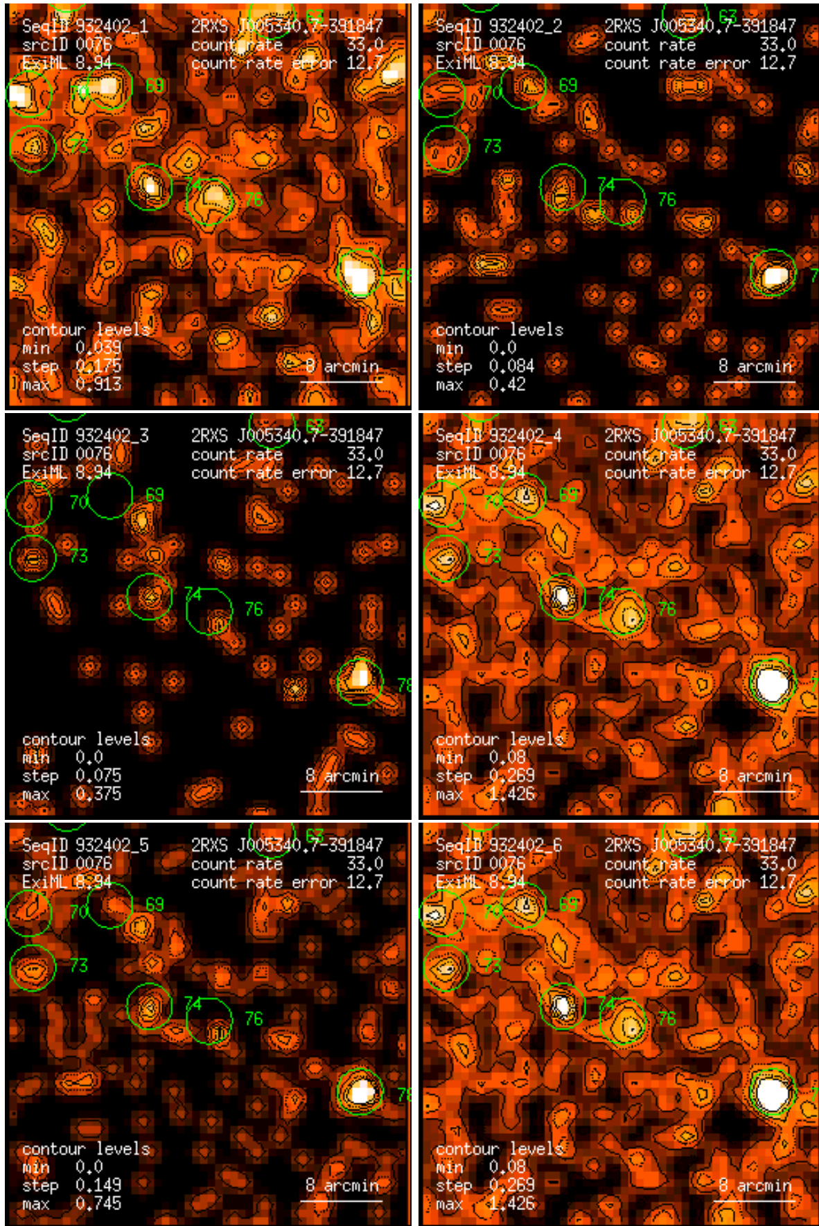
Figure 76: RASS 932402: detection 0076: band rate images, Gaussian filter: (1) PSPC channels 11 – 41, (2) 52 – 90, (3) 91 – 201, (4) 11 – 235, (5) 52 – 201, (6) 11 – 201. Broad band rates in counts/ks. Band rate contour levels in counts/ks/arcmin 2 .
