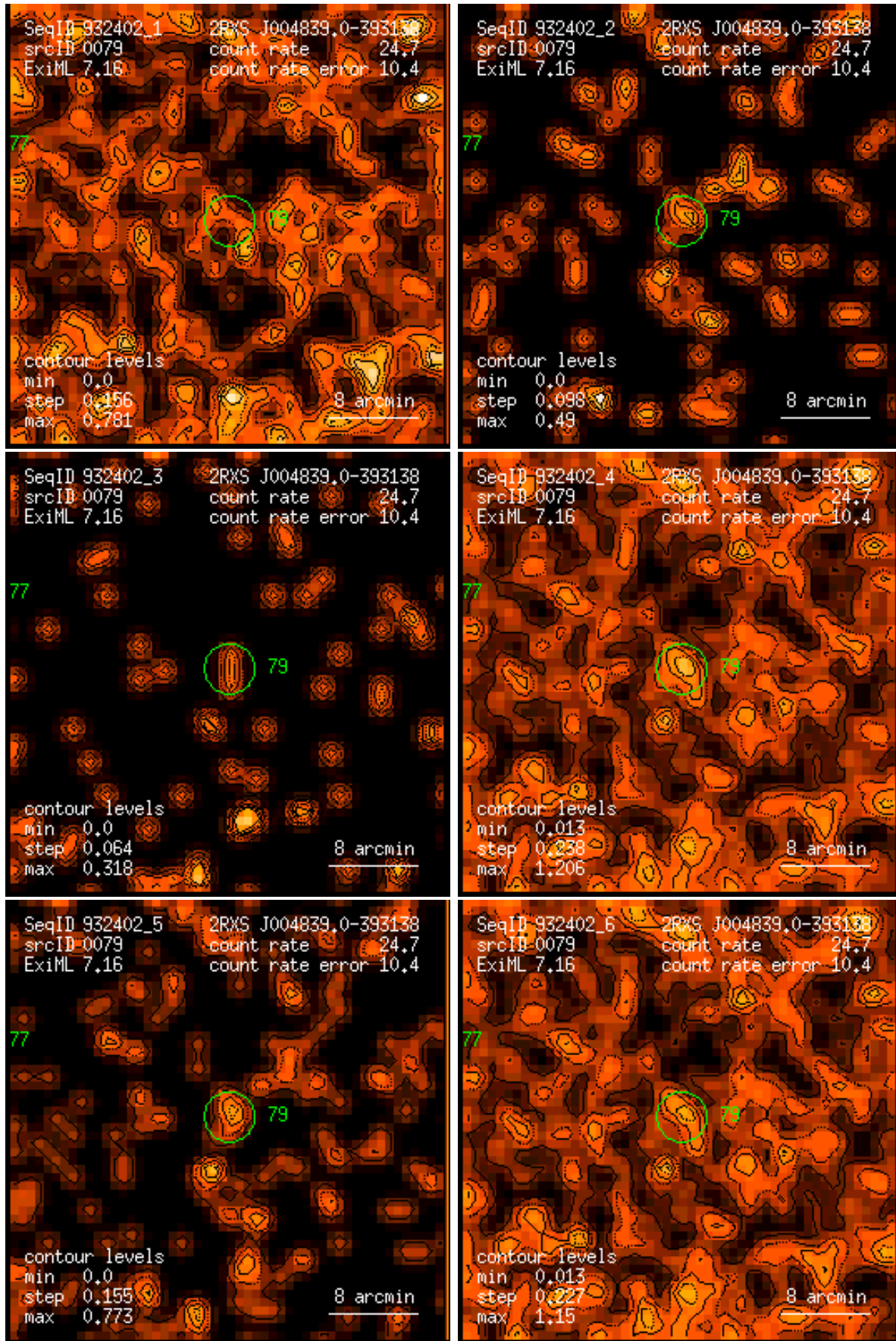
Figure 79: RASS 932402: detection 0079: band rate images, Gaussian filter: (1) PSPC channels 11 – 41, (2) 52 – 90, (3) 91 – 201, (4) 11 – 235, (5) 52 – 201, (6) 11 – 201. Broad band rates in counts/ks. Band rate contour levels in counts/ks/arcmin 2 .
