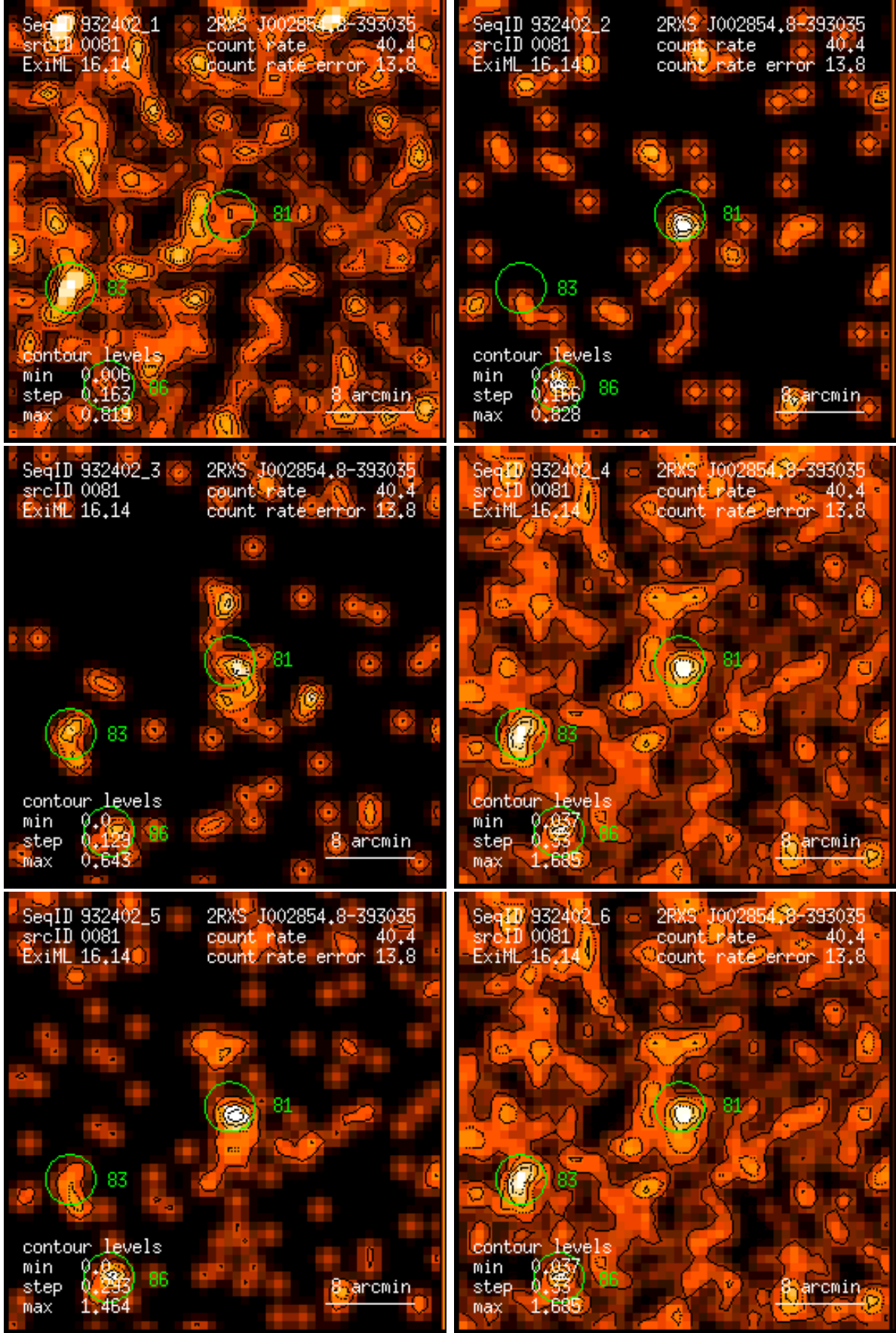
Figure 81: RASS 932402: detection 0081: band rate images, Gaussian filter: (1) PSPC channels 11 – 41, (2) 52 – 90, (3) 91 – 201, (4) 11 – 235, (5) 52 – 201, (6) 11 – 201. Broad band rates in counts/ks. Band rate contour levels in counts/ks/arcmin 2 .
