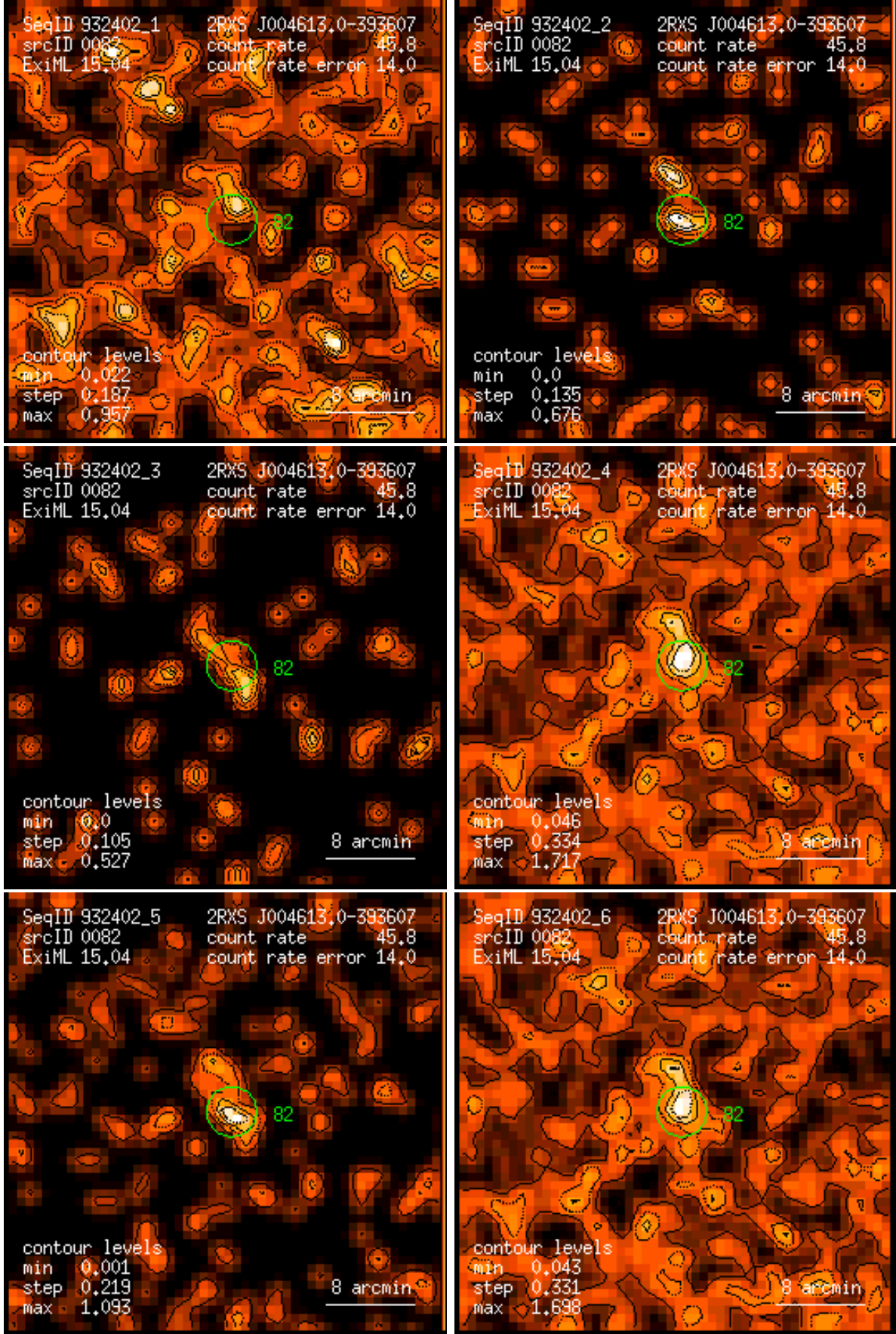
Figure 82: RASS 932402: detection 0082: band rate images, Gaussian filter: (1) PSPC channels 11 – 41, (2) 52 – 90, (3) 91 – 201, (4) 11 – 235, (5) 52 – 201, (6) 11 – 201. Broad band rates in counts/ks. Band rate contour levels in counts/ks/arcmin 2 .
