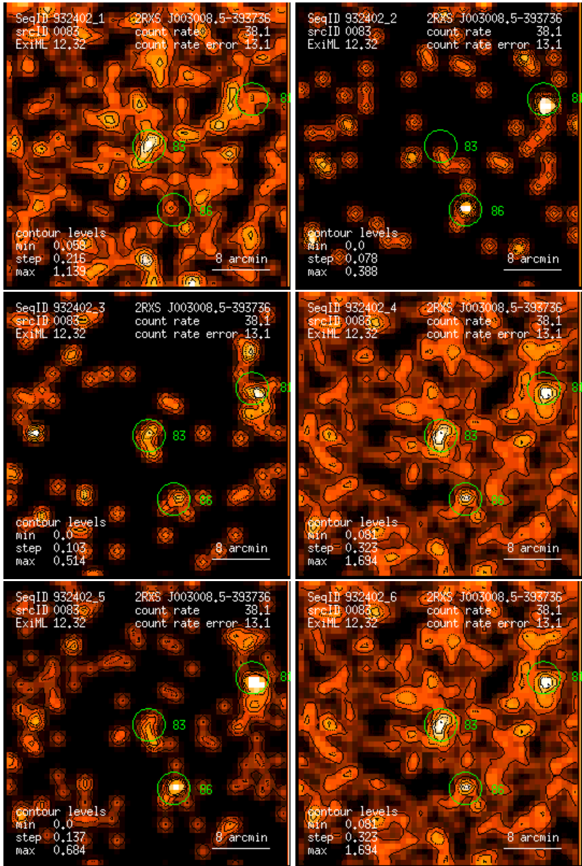
Figure 83: RASS 932402: detection 0083: band rate images, Gaussian filter: (1) PSPC channels 11 – 41, (2) 52 – 90, (3) 91 – 201, (4) 11 – 235, (5) 52 – 201, (6) 11 – 201. Broad band rates in counts/ks. Band rate contour levels in counts/ks/arcmin 2 .
