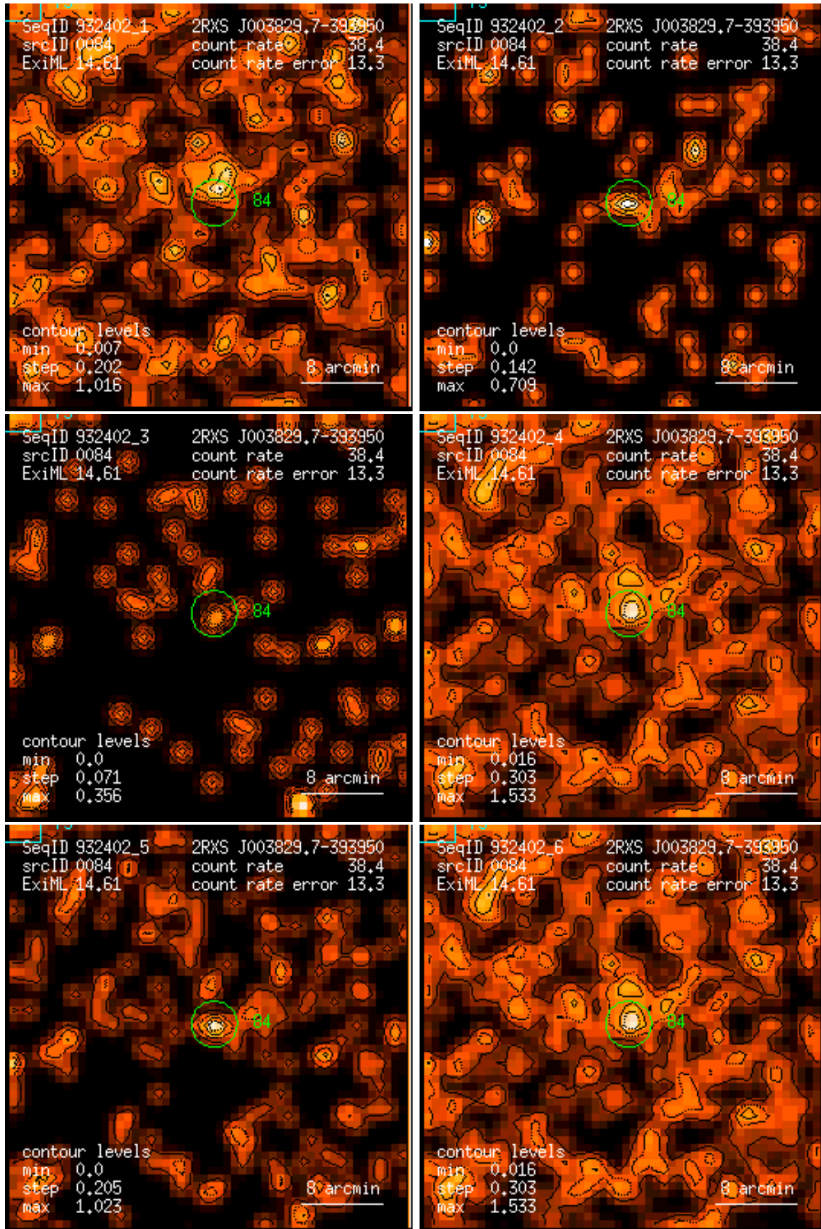
Figure 84: RASS 932402: detection 0084: band rate images, Gaussian filter: (1) PSPC channels 11 – 41, (2) 52 – 90, (3) 91 – 201, (4) 11 – 235, (5) 52 – 201, (6) 11 – 201. Broad band rates in counts/ks. Band rate contour levels in counts/ks/arcmin 2 .
