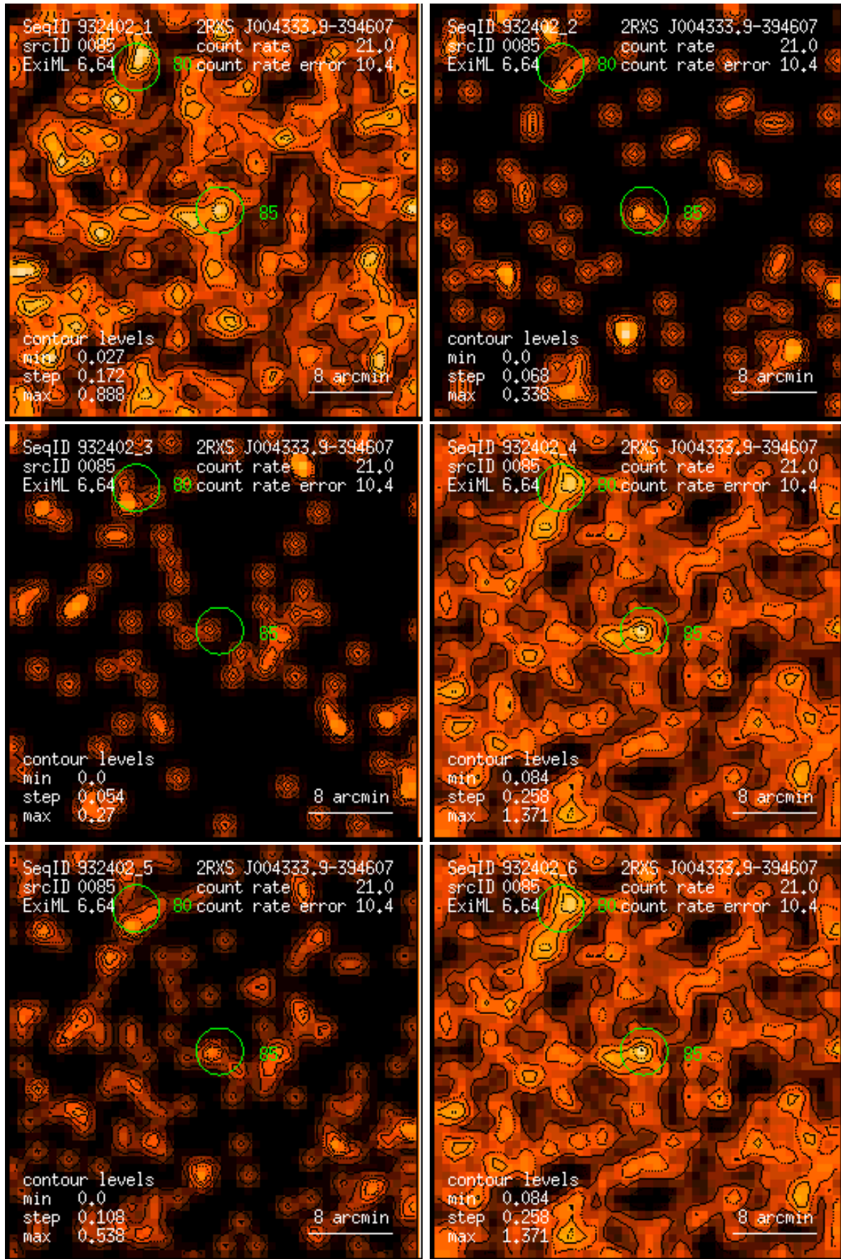
Figure 85: RASS 932402: detection 0085: band rate images, Gaussian filter: (1) PSPC channels 11 – 41, (2) 52 – 90, (3) 91 – 201, (4) 11 – 235, (5) 52 – 201, (6) 11 – 201. Broad band rates in counts/ks. Band rate contour levels in counts/ks/arcmin 2 .
