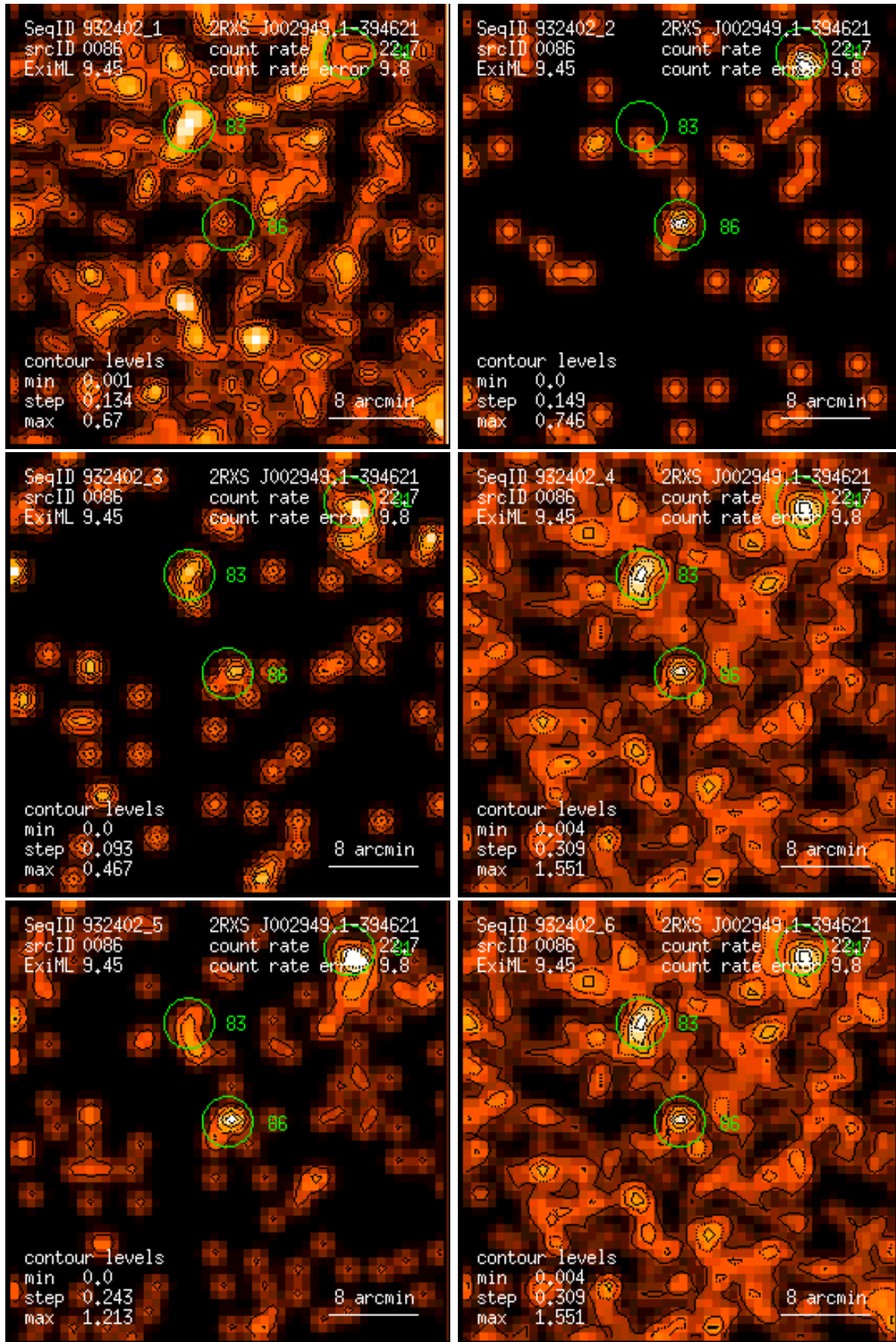
Figure 86: RASS 932402: detection 0086: band rate images, Gaussian filter: (1) PSPC channels 11 – 41, (2) 52 – 90, (3) 91 – 201, (4) 11 – 235, (5) 52 – 201, (6) 11 – 201. Broad band rates in counts/ks. Band rate contour levels in counts/ks/arcmin 2 .
