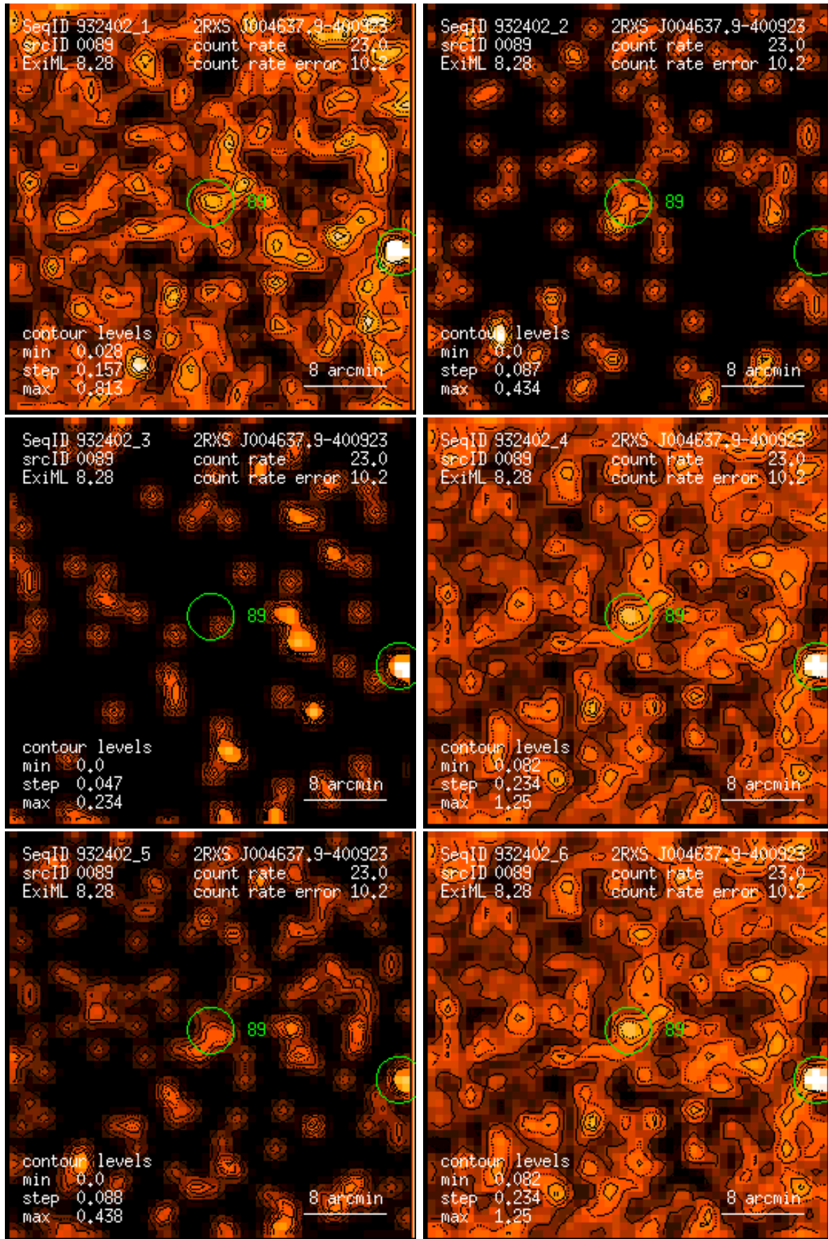
Figure 89: RASS 932402: detection 0089: band rate images, Gaussian filter: (1) PSPC channels 11 – 41, (2) 52 – 90, (3) 91 – 201, (4) 11 – 235, (5) 52 – 201, (6) 11 – 201. Broad band rates in counts/ks. Band rate contour levels in counts/ks/arcmin 2 .
