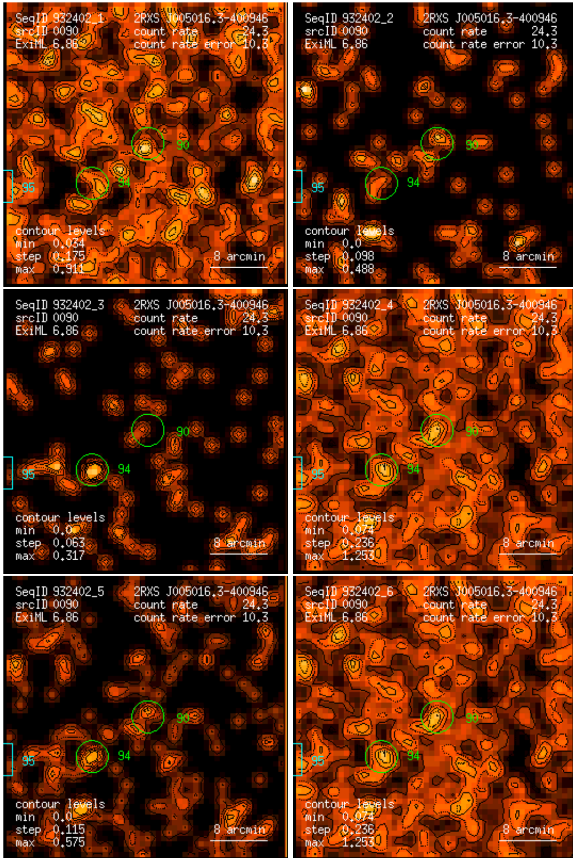
Figure 90: RASS 932402: detection 0090: band rate images, Gaussian filter: (1) PSPC channels 11 – 41, (2) 52 – 90, (3) 91 – 201, (4) 11 – 235, (5) 52 – 201, (6) 11 – 201. Broad band rates in counts/ks. Band rate contour levels in counts/ks/arcmin 2 .
