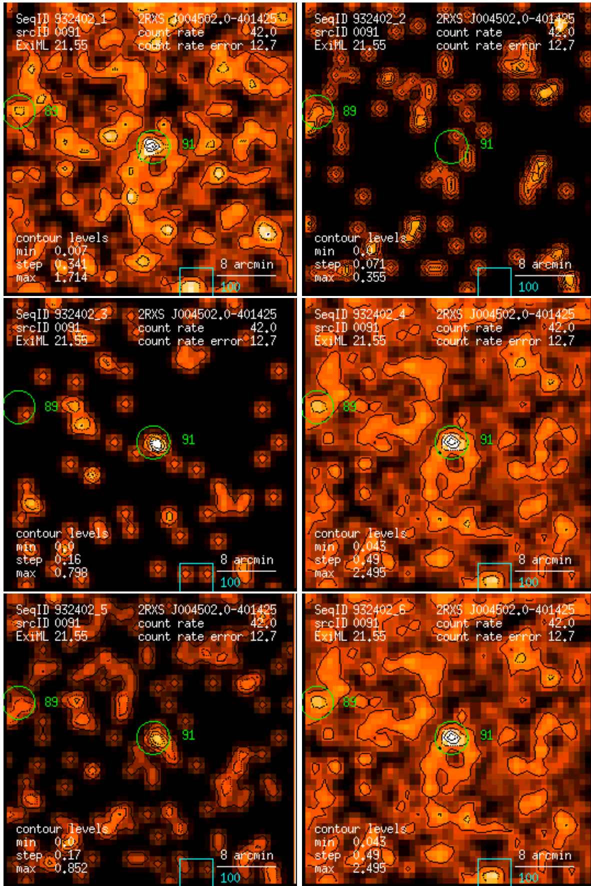
Figure 91: RASS 932402: detection 0091: band rate images, Gaussian filter: (1) PSPC channels 11 – 41, (2) 52 – 90, (3) 91 – 201, (4) 11 – 235, (5) 52 – 201, (6) 11 – 201. Broad band rates in counts/ks. Band rate contour levels in counts/ks/arcmin 2 .
