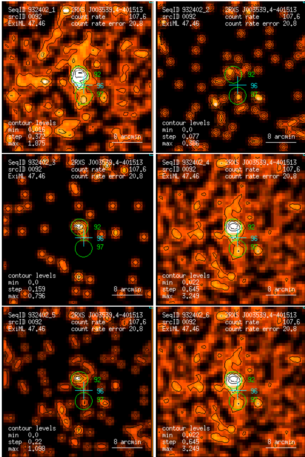
Figure 92: RASS 932402: detection 0092: band rate images, Gaussian filter: (1) PSPC channels 11 – 41, (2) 52 – 90, (3) 91 – 201, (4) 11 – 235, (5) 52 – 201, (6) 11 – 201. Broad band rates in counts/ks. Band rate contour levels in counts/ks/arcmin 2 .
