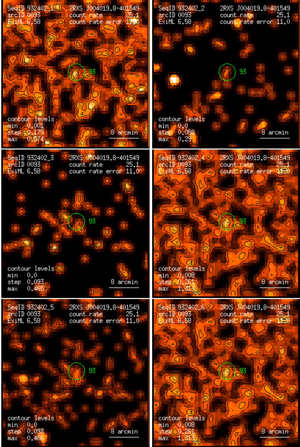
Figure 93: RASS 932402: detection 0093: band rate images, Gaussian filter: (1) PSPC channels 11 – 41, (2) 52 – 90, (3) 91 – 201, (4) 11 – 235, (5) 52 – 201, (6) 11 – 201. Broad band rates in counts/ks. Band rate contour levels in counts/ks/arcmin 2 .
