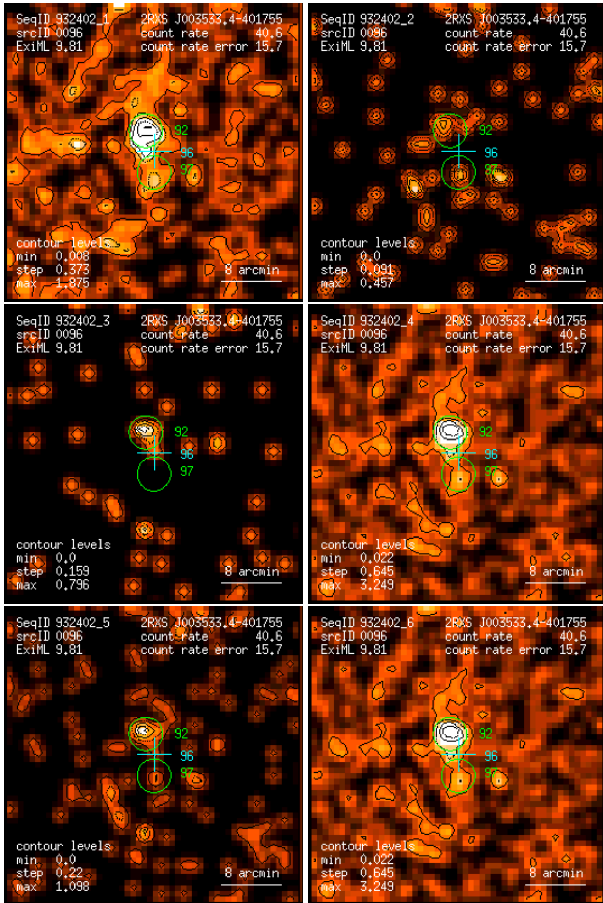
Figure 96: RASS 932402: detection 0096: band rate images, Gaussian filter: (1) PSPC channels 11 – 41, (2) 52 – 90, (3) 91 – 201, (4) 11 – 235, (5) 52 – 201, (6) 11 – 201. Broad band rates in counts/ks. Band rate contour levels in counts/ks/arcmin 2 .
