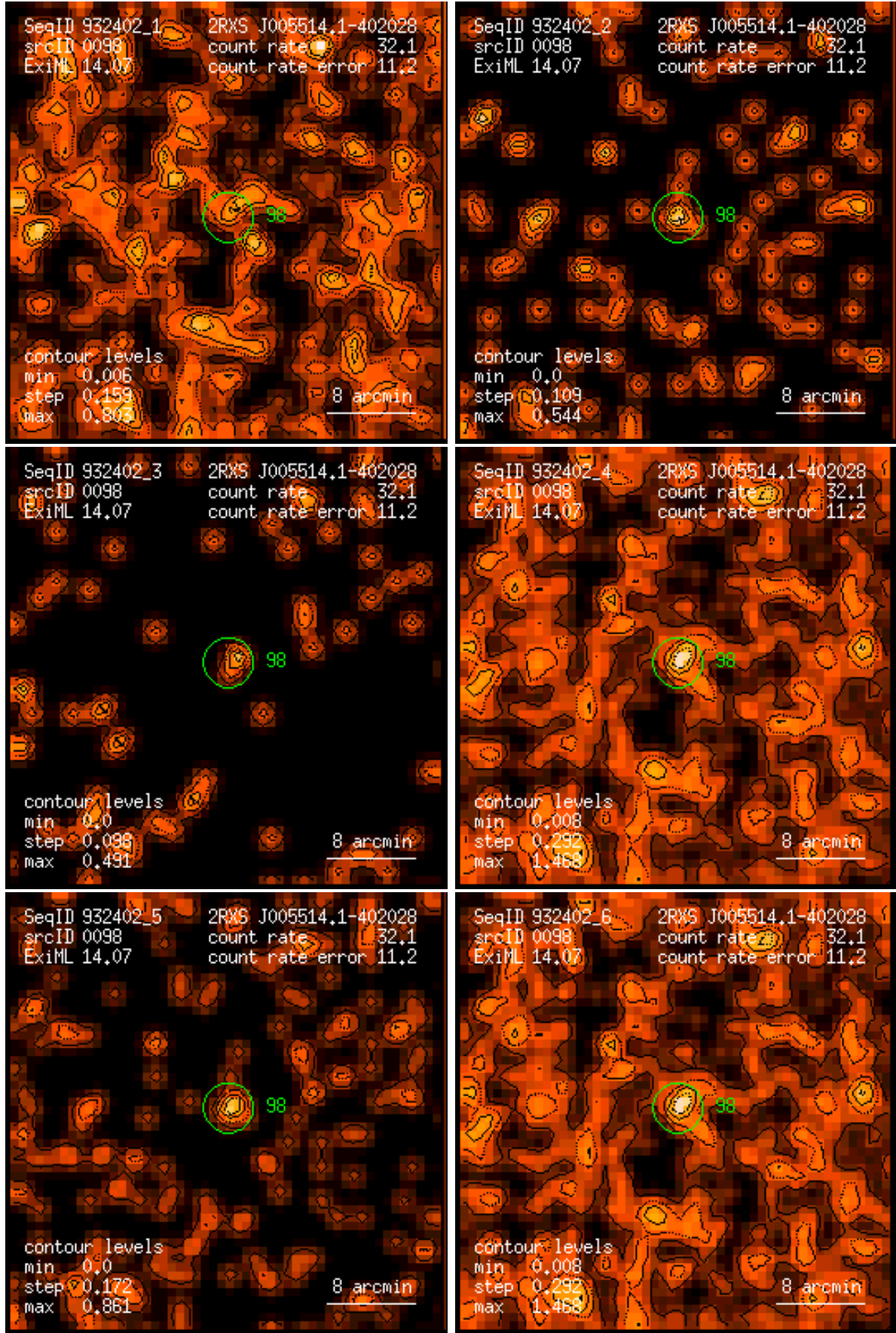
Figure 98: RASS 932402: detection 0098: band rate images, Gaussian filter: (1) PSPC channels 11 – 41, (2) 52 – 90, (3) 91 – 201, (4) 11 – 235, (5) 52 – 201, (6) 11 – 201. Broad band rates in counts/ks. Band rate contour levels in counts/ks/arcmin 2 .
