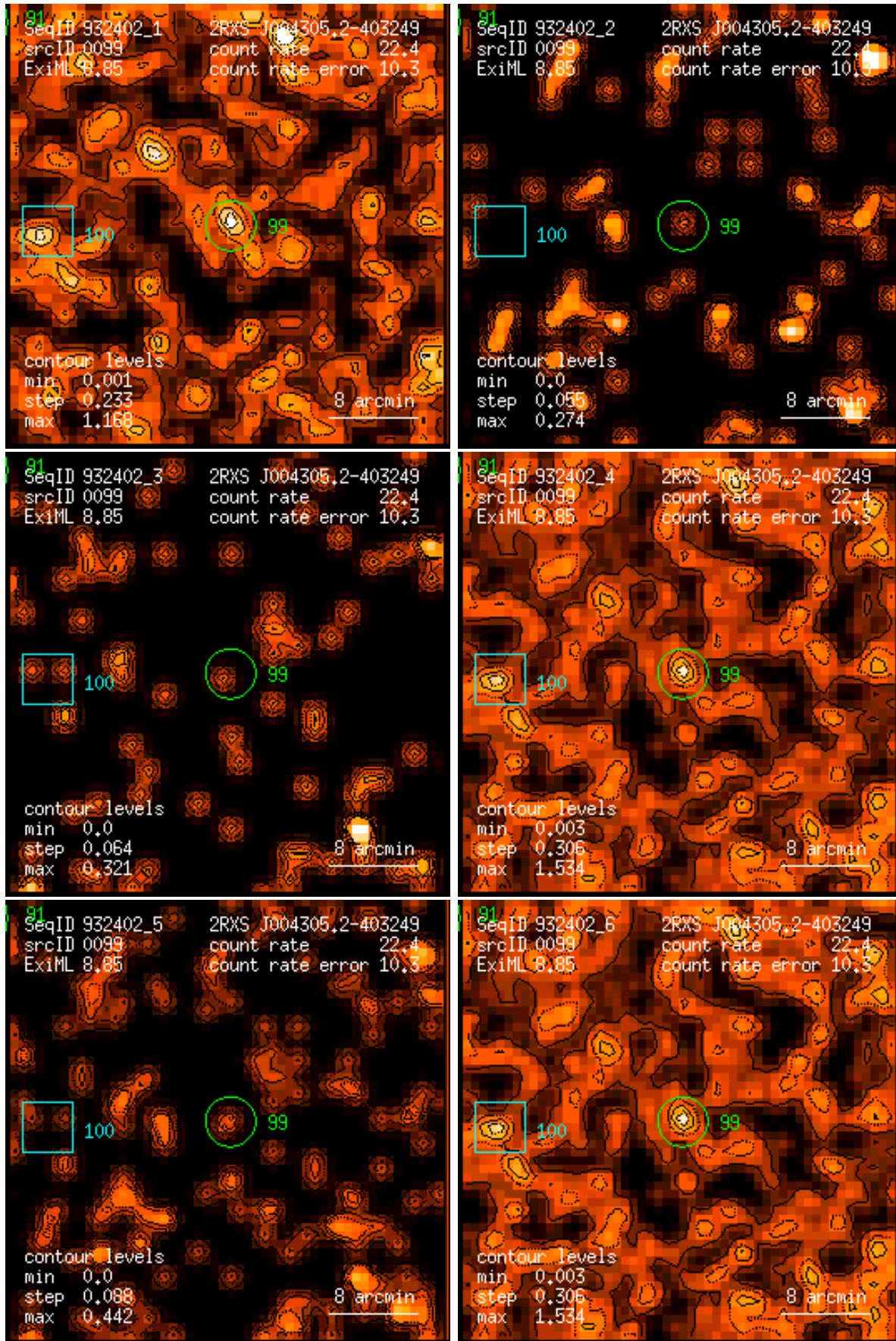
Figure 99: RASS 932402: detection 0099: band rate images, Gaussian filter: (1) PSPC channels 11 – 41, (2) 52 – 90, (3) 91 – 201, (4) 11 – 235, (5) 52 – 201, (6) 11 – 201. Broad band rates in counts/ks. Band rate contour levels in counts/ks/arcmin 2 .
