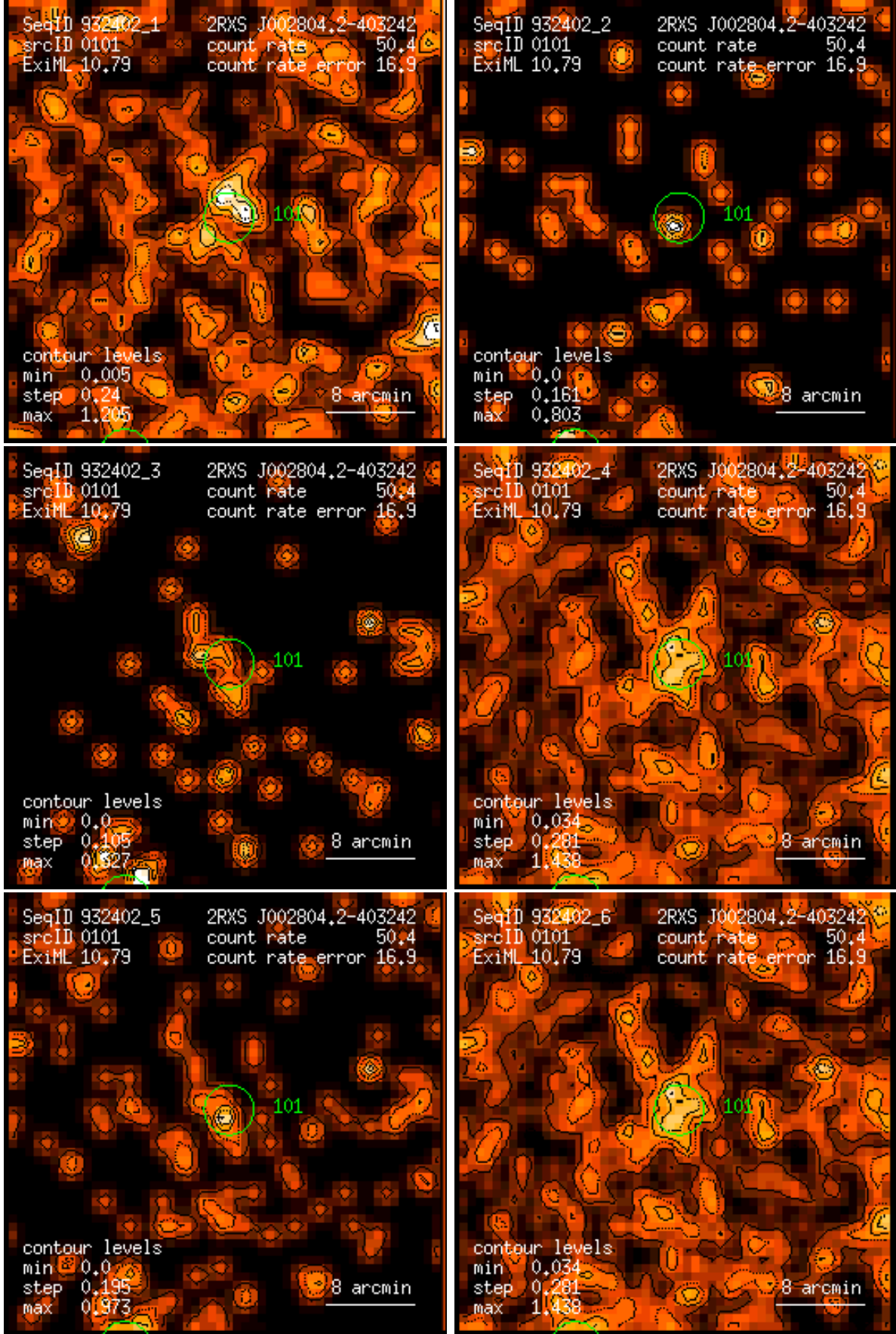
Figure 101: RASS 932402: detection 0101: band rate images, Gaussian filter: (1) PSPC channels 11 – 41, (2) 52 – 90, (3) 91 – 201, (4) 11 – 235, (5) 52 – 201, (6) 11 – 201. Broad band rates in counts/ks. Band rate contour levels in counts/ks/arcmin 2 .
