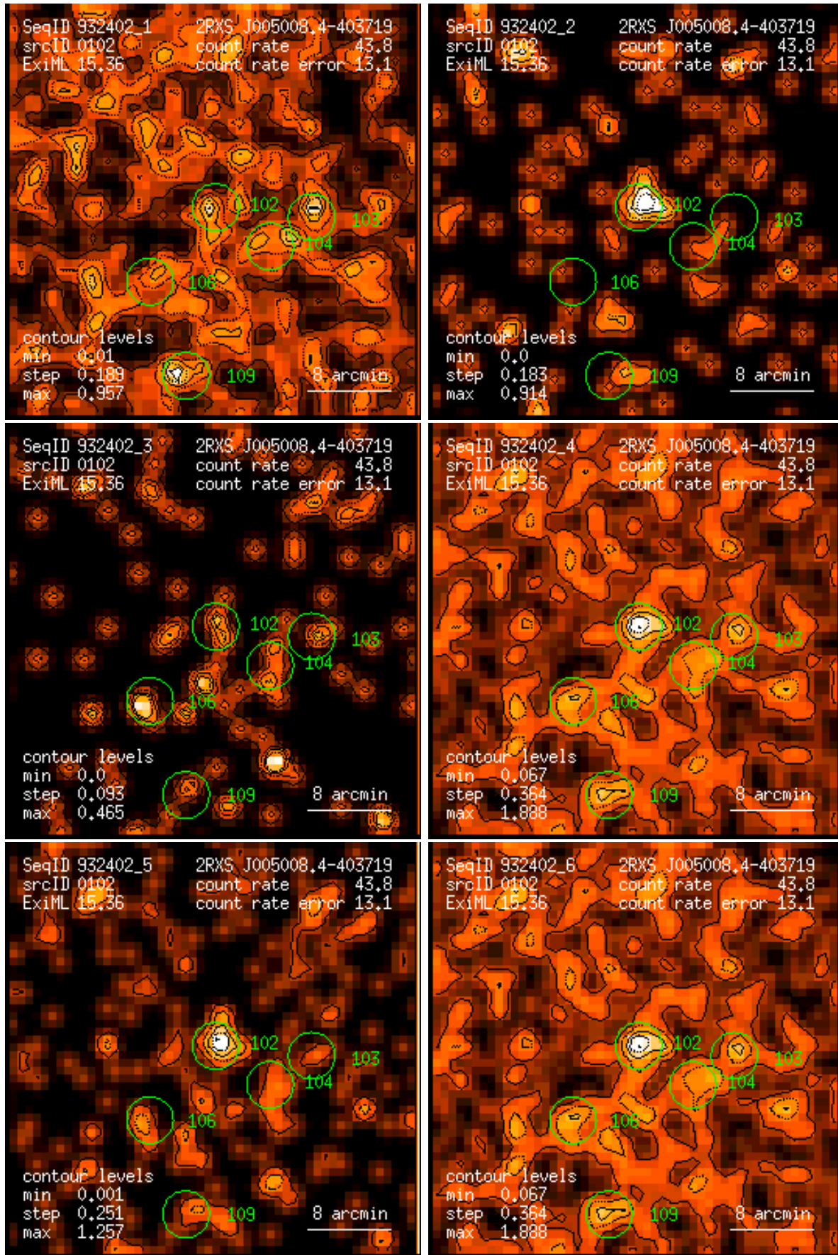
Figure 102: RASS 932402: detection 0102: band rate images, Gaussian filter: (1) PSPC channels 11 – 41, (2) 52 – 90, (3) 91 – 201, (4) 11 – 235, (5) 52 – 201, (6) 11 – 201. Broad band rates in counts/ks. Band rate contour levels in counts/ks/arcmin 2 .
