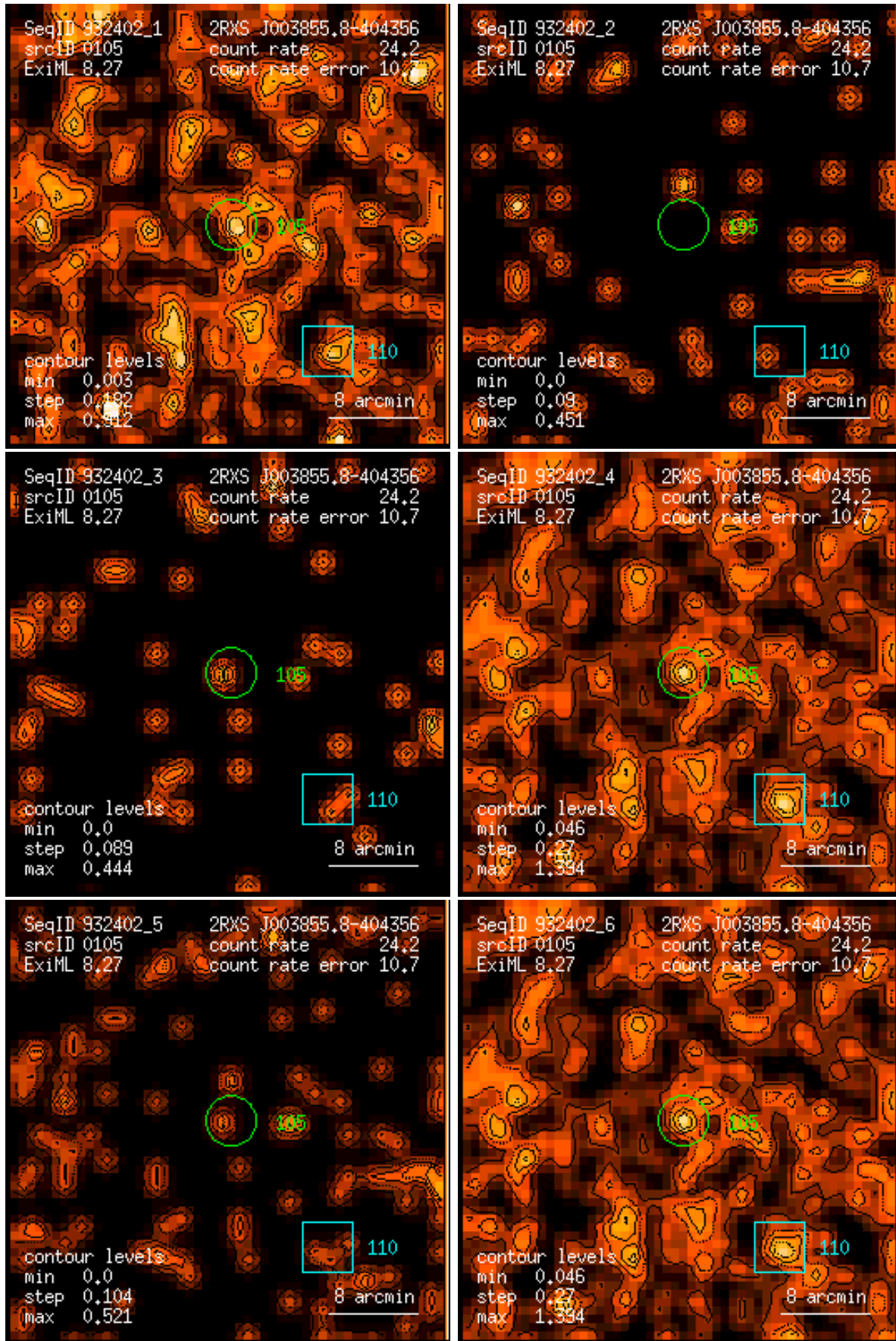
Figure 105: RASS 932402: detection 0105: band rate images, Gaussian filter: (1) PSPC channels 11 – 41, (2) 52 – 90, (3) 91 – 201, (4) 11 – 235, (5) 52 – 201, (6) 11 – 201. Broad band rates in counts/ks. Band rate contour levels in counts/ks/arcmin 2 .
