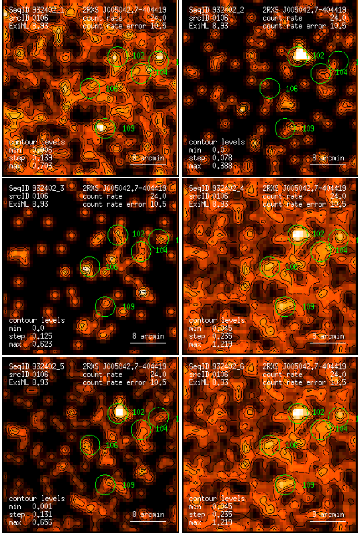
Figure 106: RASS 932402: detection 0106: band rate images, Gaussian filter: (1) PSPC channels 11 – 41, (2) 52 – 90, (3) 91 – 201, (4) 11 – 235, (5) 52 – 201, (6) 11 – 201. Broad band rates in counts/ks. Band rate contour levels in counts/ks/arcmin 2 .
