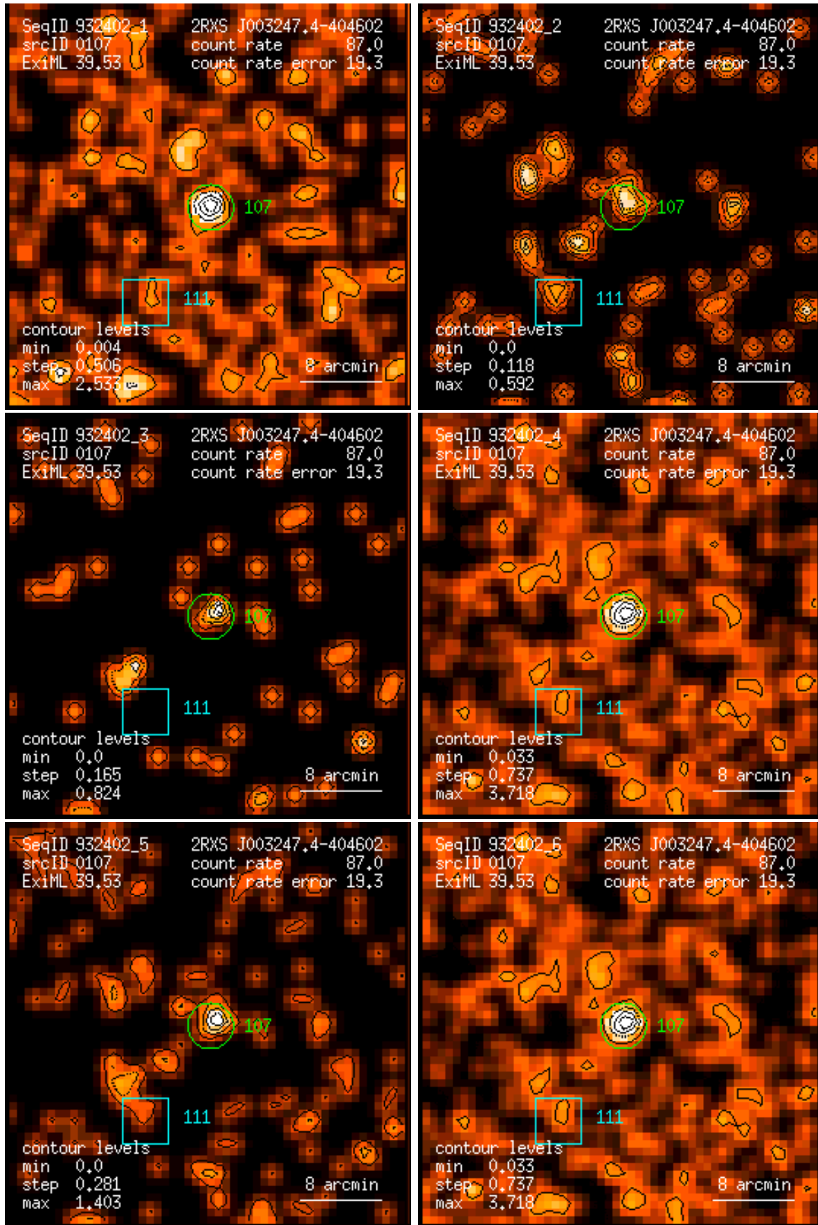
Figure 107: RASS 932402: detection 0107: band rate images, Gaussian filter: (1) PSPC channels 11 – 41, (2) 52 – 90, (3) 91 – 201, (4) 11 – 235, (5) 52 – 201, (6) 11 – 201. Broad band rates in counts/ks. Band rate contour levels in counts/ks/arcmin 2 .
