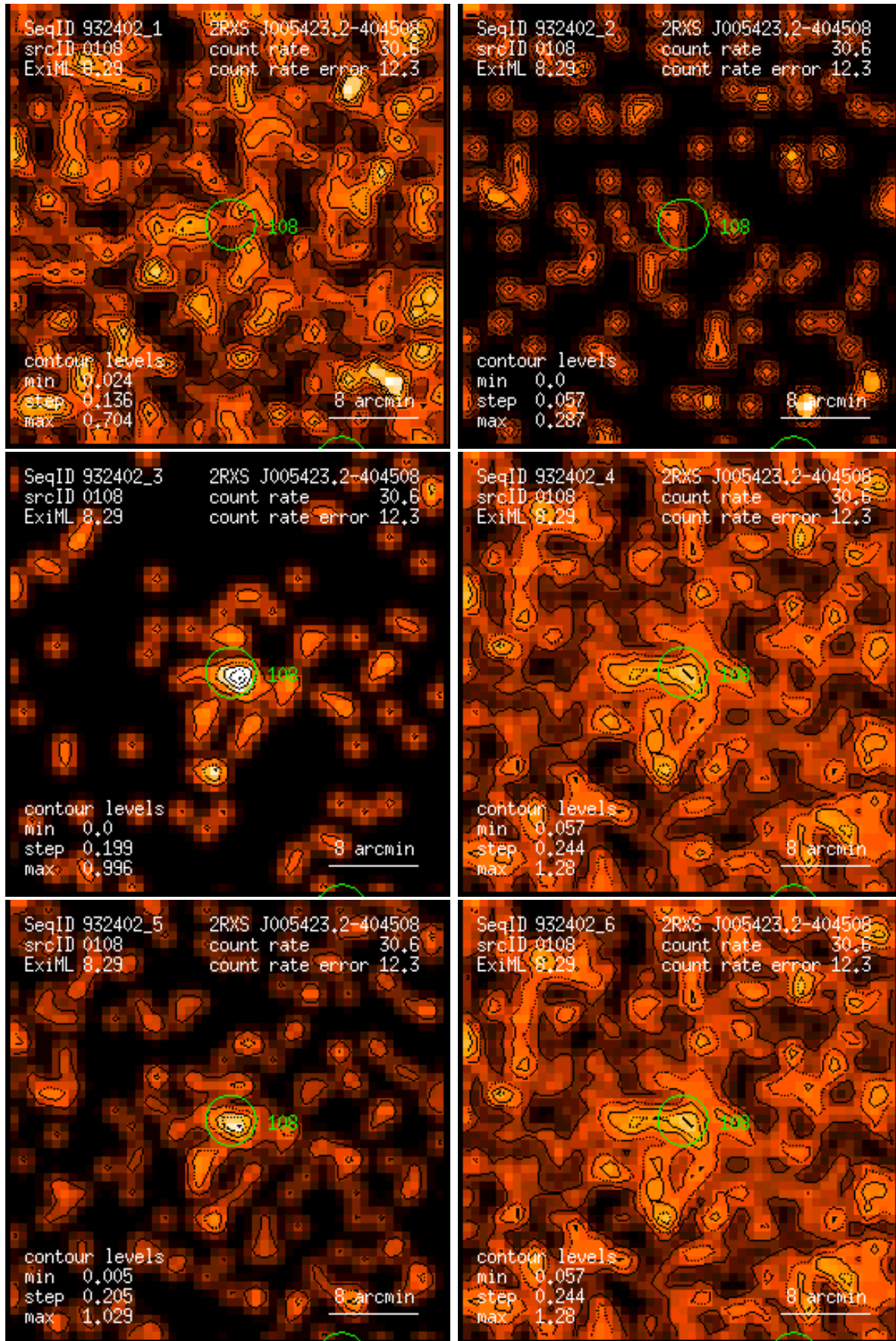
Figure 108: RASS 932402: detection 0108: band rate images, Gaussian filter: (1) PSPC channels 11 – 41, (2) 52 – 90, (3) 91 – 201, (4) 11 – 235, (5) 52 – 201, (6) 11 – 201. Broad band rates in counts/ks. Band rate contour levels in counts/ks/arcmin 2 .
