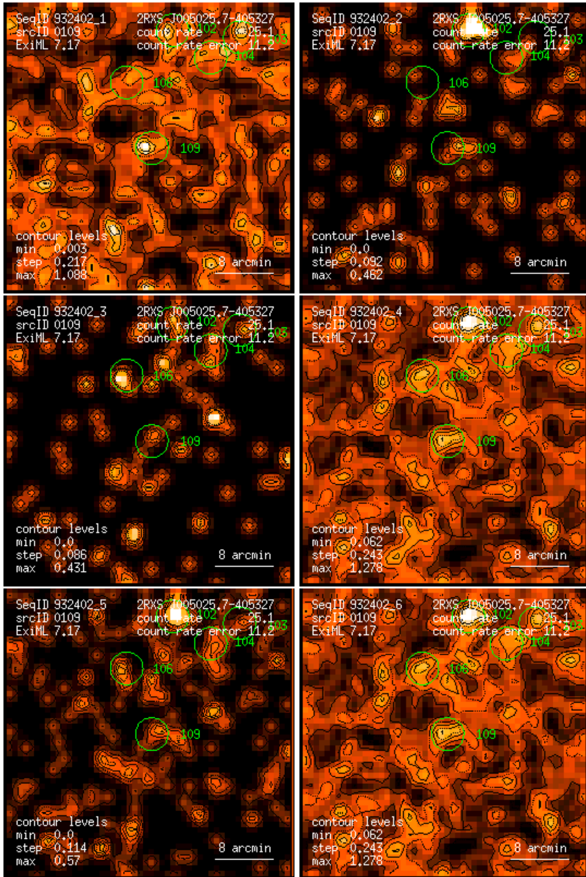
Figure 109: RASS 932402: detection 0109: band rate images, Gaussian filter: (1) PSPC channels 11 – 41, (2) 52 – 90, (3) 91 – 201, (4) 11 – 235, (5) 52 – 201, (6) 11 – 201. Broad band rates in counts/ks. Band rate contour levels in counts/ks/arcmin 2 .
