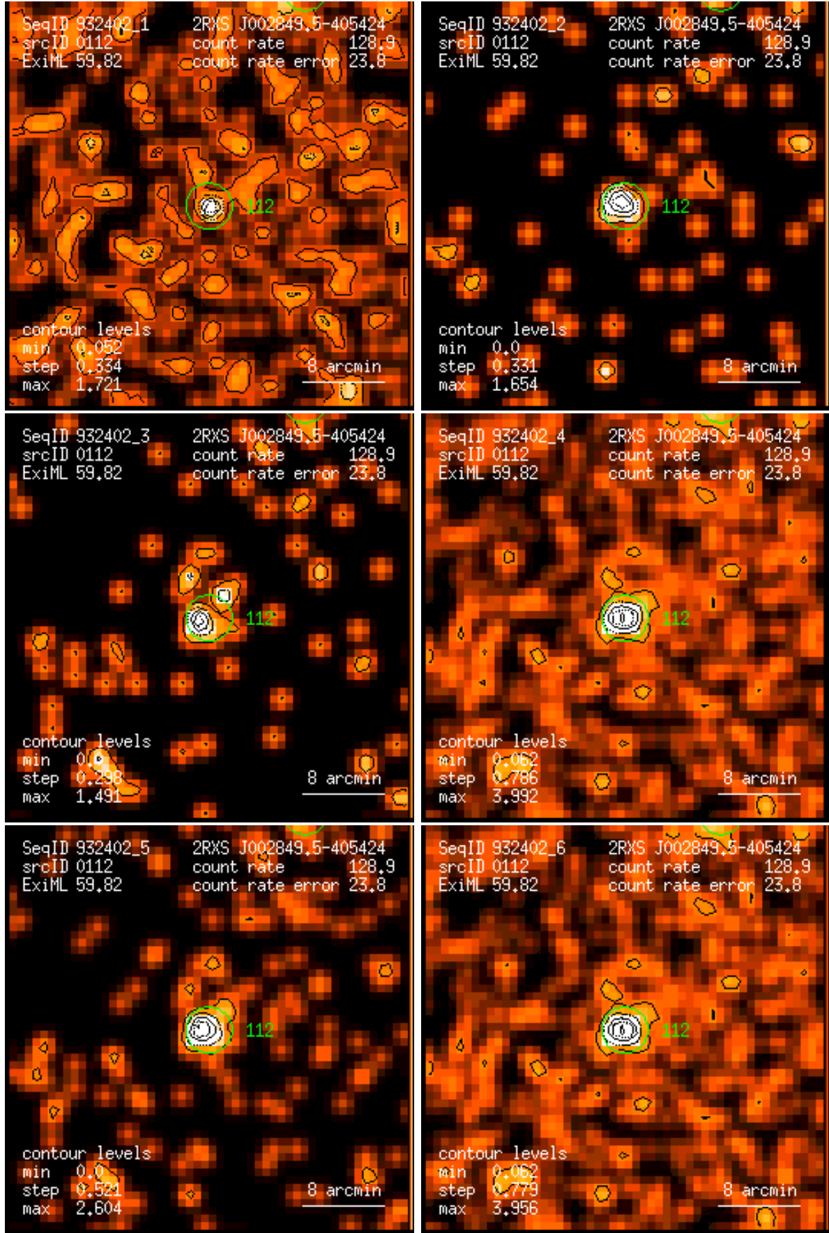
Figure 112: RASS 932402: detection 0112: band rate images, Gaussian filter: (1) PSPC channels 11 – 41, (2) 52 – 90, (3) 91 – 201, (4) 11 – 235, (5) 52 – 201, (6) 11 – 201. Broad band rates in counts/ks. Band rate contour levels in counts/ks/arcmin 2 .
