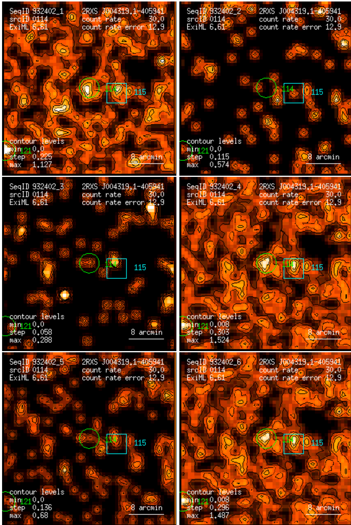
Figure 114: RASS 932402: detection 0114: band rate images, Gaussian filter: (1) PSPC channels 11 – 41, (2) 52 – 90, (3) 91 – 201, (4) 11 – 235, (5) 52 – 201, (6) 11 – 201. Broad band rates in counts/ks. Band rate contour levels in counts/ks/arcmin 2 .
