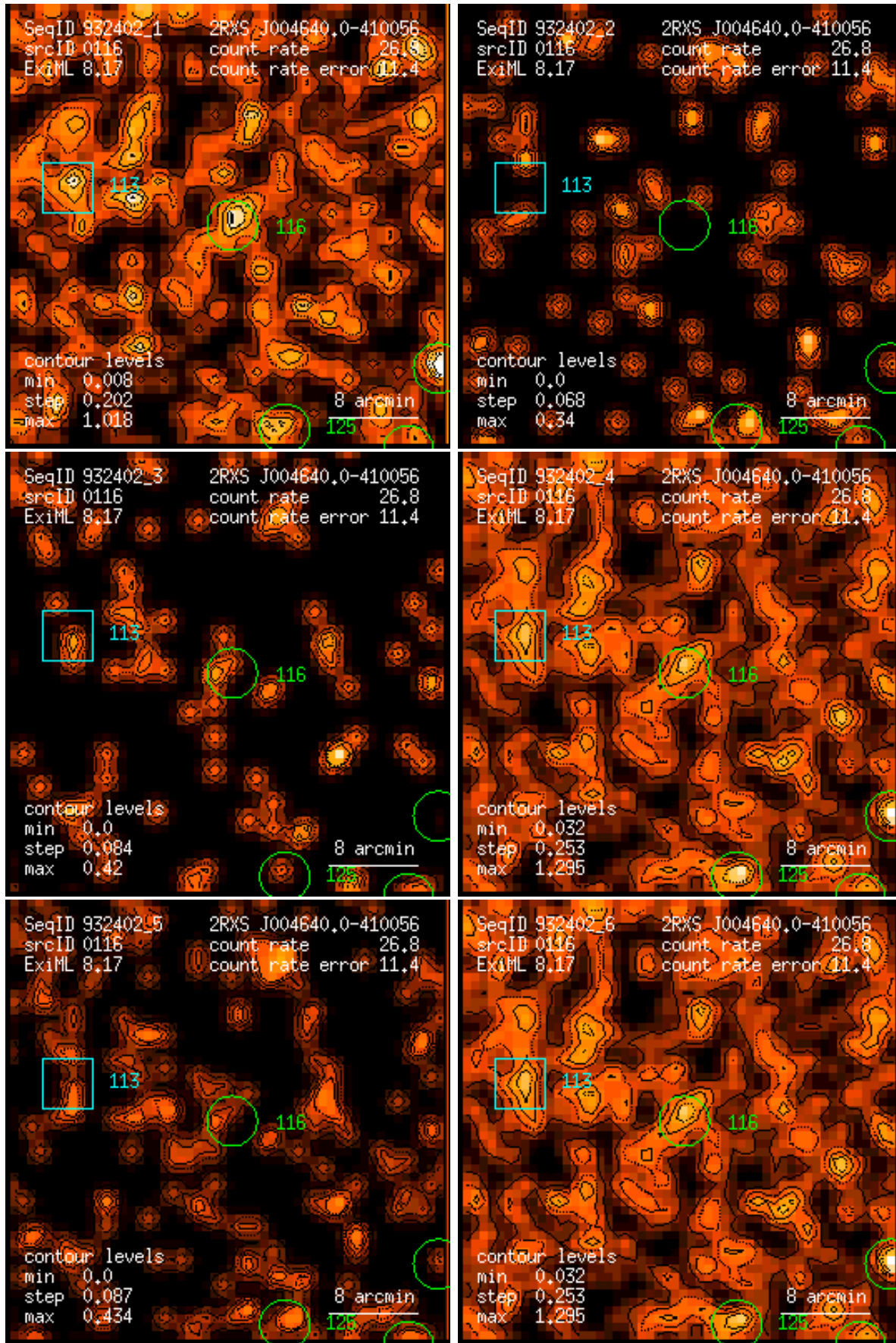
Figure 116: RASS 932402: detection 0116: band rate images, Gaussian filter: (1) PSPC channels 11 – 41, (2) 52 – 90, (3) 91 – 201, (4) 11 – 235, (5) 52 – 201, (6) 11 – 201. Broad band rates in counts/ks. Band rate contour levels in counts/ks/arcmin 2 .
