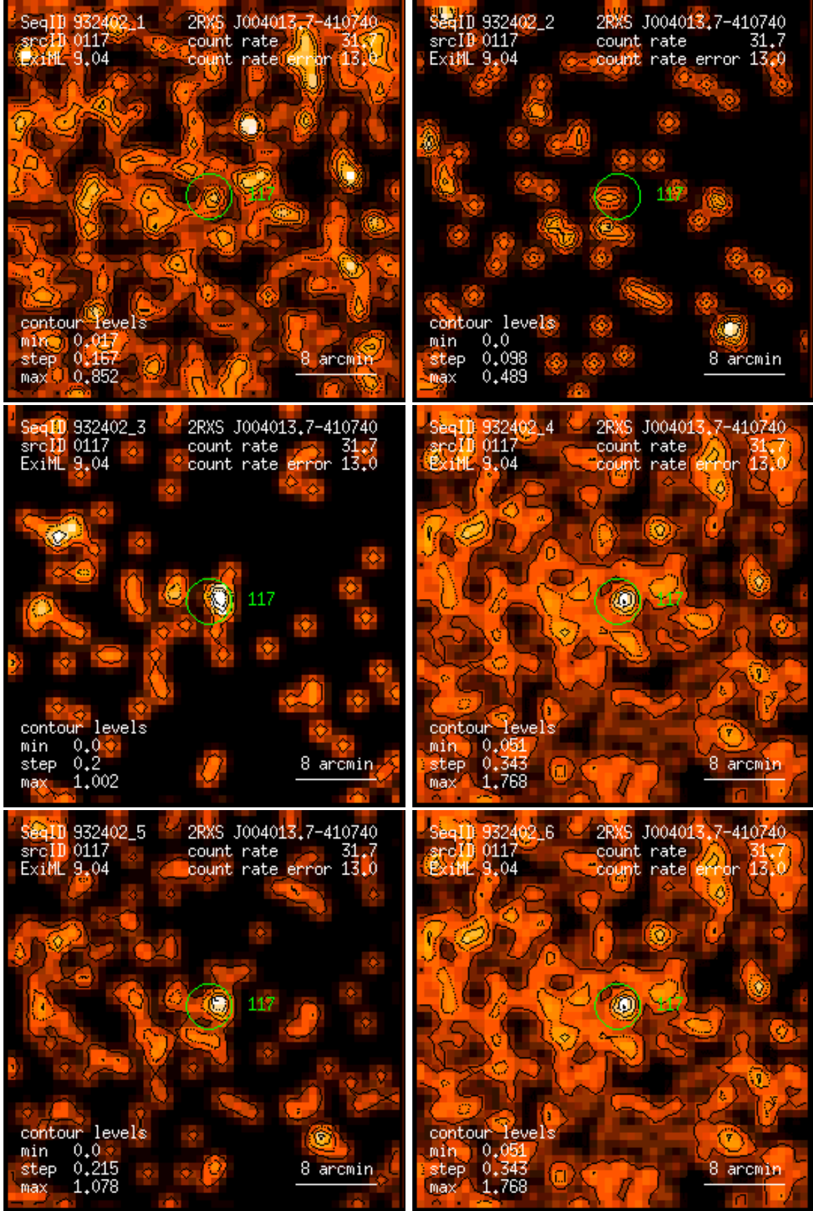
Figure 117: RASS 932402: detection 0117: band rate images, Gaussian filter: (1) PSPC channels 11 – 41, (2) 52 – 90, (3) 91 – 201, (4) 11 – 235, (5) 52 – 201, (6) 11 – 201. Broad band rates in counts/ks. Band rate contour levels in counts/ks/arcmin 2 .
