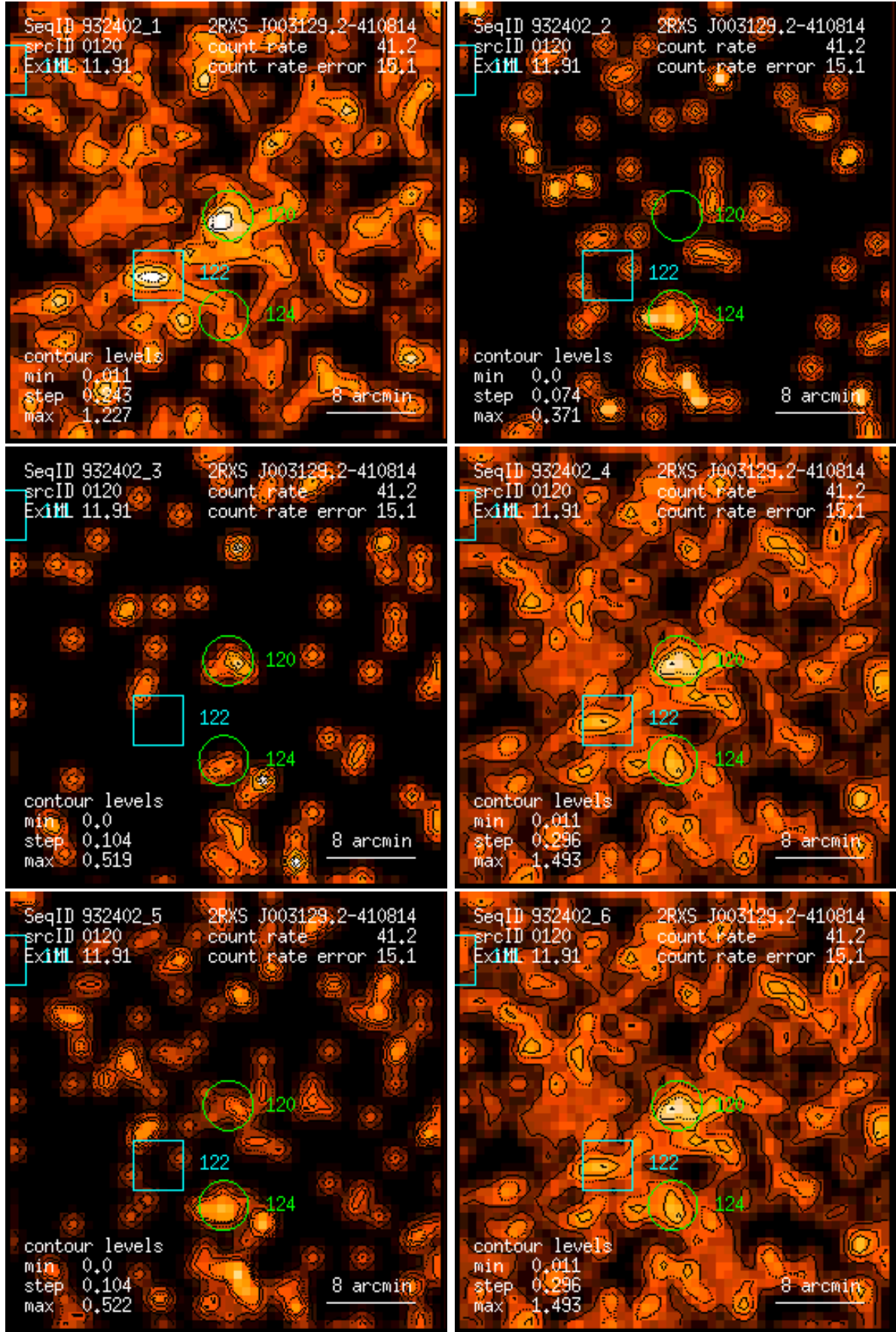
Figure 120: RASS 932402: detection 0120: band rate images, Gaussian filter: (1) PSPC channels 11 – 41, (2) 52 – 90, (3) 91 – 201, (4) 11 – 235, (5) 52 – 201, (6) 11 – 201. Broad band rates in counts/ks. Band rate contour levels in counts/ks/arcmin 2 .
