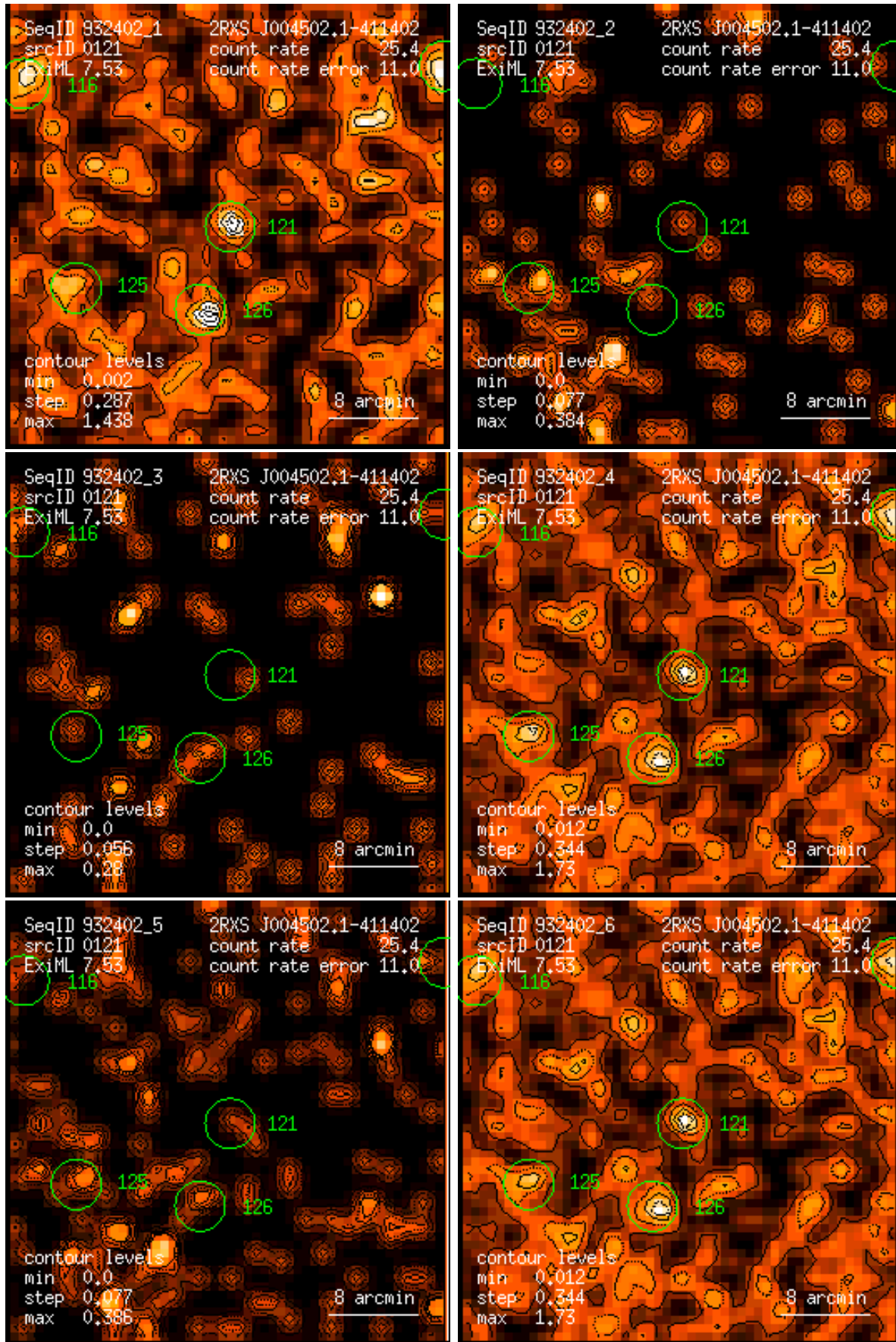
Figure 121: RASS 932402: detection 0121: band rate images, Gaussian filter: (1) PSPC channels 11 – 41, (2) 52 – 90, (3) 91 – 201, (4) 11 – 235, (5) 52 – 201, (6) 11 – 201. Broad band rates in counts/ks. Band rate contour levels in counts/ks/arcmin 2 .
