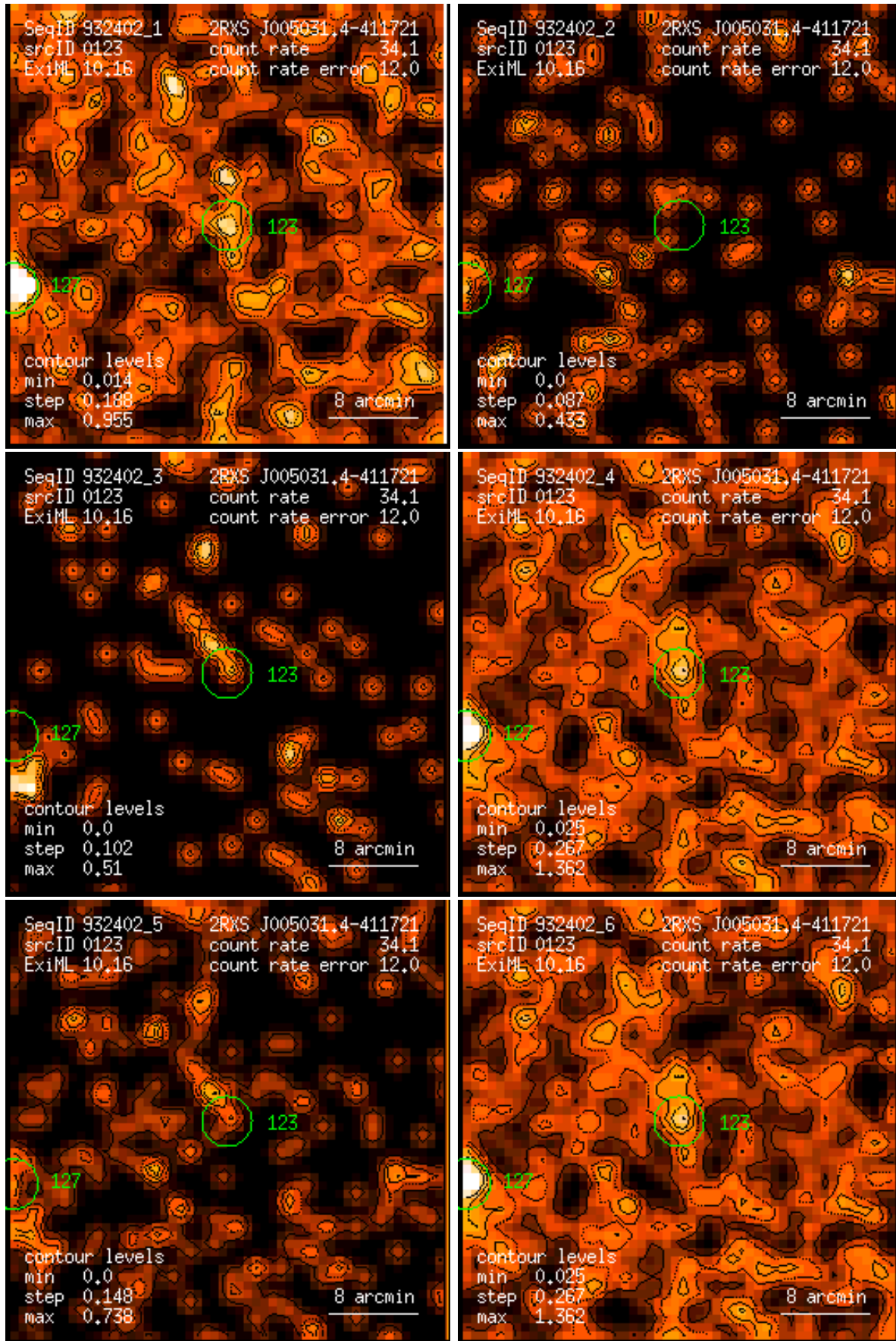
Figure 123: RASS 932402: detection 0123: band rate images, Gaussian filter: (1) PSPC channels 11 – 41, (2) 52 – 90, (3) 91 – 201, (4) 11 – 235, (5) 52 – 201, (6) 11 – 201. Broad band rates in counts/ks. Band rate contour levels in counts/ks/arcmin 2 .
